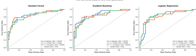
Fig. 11. ROC curves by classifier and training scenario on the 83-patient real held-out test set: Random Forest (left), Gradient Boosting (centre), Logistic Regression (right). All curves lie substantially above the random classifier diagonal. Gradient Boosting under Scenario A achieves the highest AUC at 0.878. Scenario D (SMOTE) achieves the highest overall accuracy at 0.807 under Gradient Boosting.
