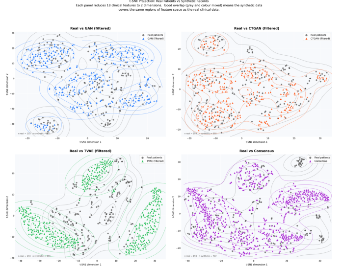
Fig. 9. t-SNE two-dimensional projection of real patients and each synthetic method in the original 18-dimensional feature space. GAN and CTGAN filtered sets show reasonable overlap with the real patient manifold. TVAE points spread more widely, with portions falling outside the real patient density contours. The consensus set fills the central high-density region.
