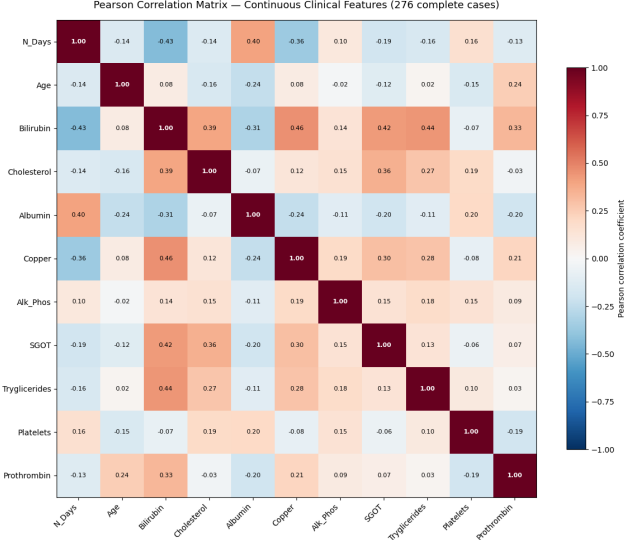
Fig. 1. Pearson correlation matrix across all 276 complete cases. Bilirubin shows strong positive correlations with Copper ( r = 0.46 ), SGOT ( r = 0.42 ), Cholesterol ( r = 0.39 ), and Prothrombin ( r = 0.33 ), reflecting the interlinked nature of hepatic synthetic and excretory function in PBC. N_Days is negatively correlated with Bilirubin ( r = -0.43 ) and Copper ( r = -0.36 ), consistent with more severe biochemical profiles being associated with shorter survival.
