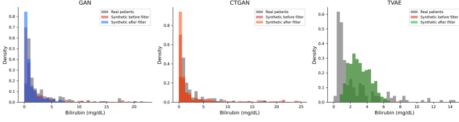
Fig. 2. Effect of IQR-based Tukey fence filtering on the Bilirubin distribution for all three generative models. Grey bars show real patient density. Pink bars show unfiltered synthetic distribution; coloured bars show the post-filter distribution. The GAN and CTGAN produce records extending beyond 15 mg/dL that the filter removes. The TVAE retains all generated records but produces a distribution shifted rightward relative to real patients.
