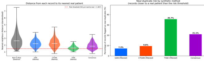
Fig. 5. Privacy disclosure risk analysis using nearest-neighbour distances in standardised feature space. Left: violin plots of distances from each synthetic record to its closest real training patient. The red dashed line marks the risk threshold at the 5th percentile of real-to-real distances. GAN and CTGAN distributions are centred above this threshold. Right: near-duplicate rates by method. GAN (7.3%) and CTGAN (9.6%) present low privacy risk, TVAE the highest at 35.7%, and the equalised consensus set 21.1%.
