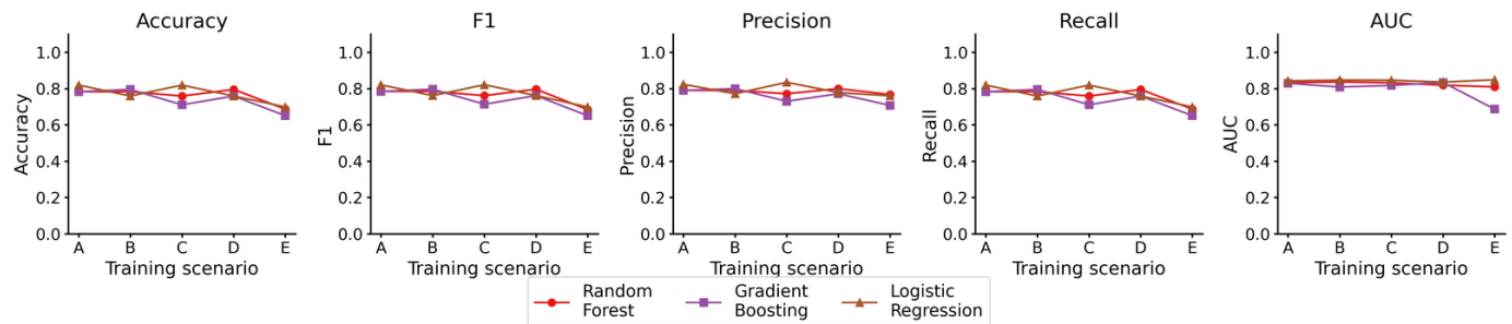
Fig. S9. Grouped comparison of accuracy, F1 and AUC across all training scenarios and classifiers. No augmentation scenario uniformly outperforms the real-data baseline.
