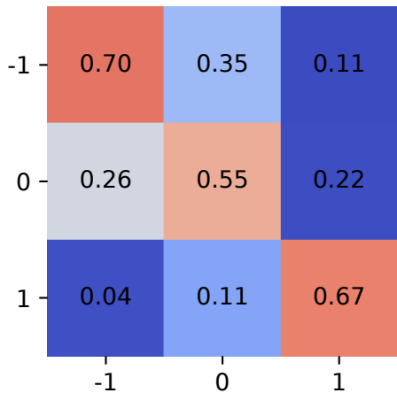
L6_CT_CTX_Glut; n = 2206
