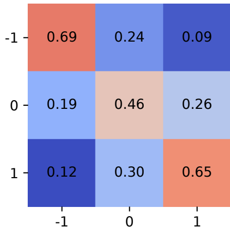
CA1-ProS_Glut; n = 1828
