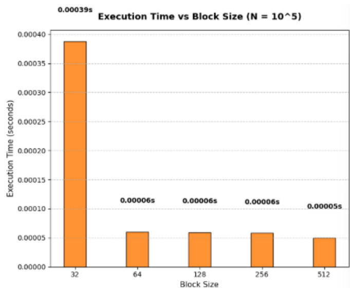
(Comparison between block sizes for N = 10 5 )
