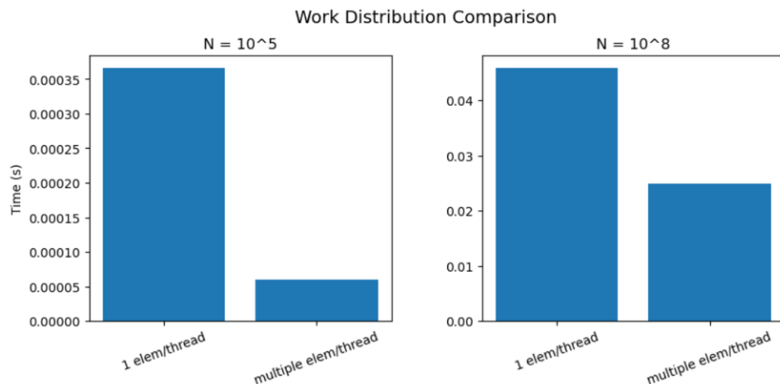
(Comparison between times for different N)
