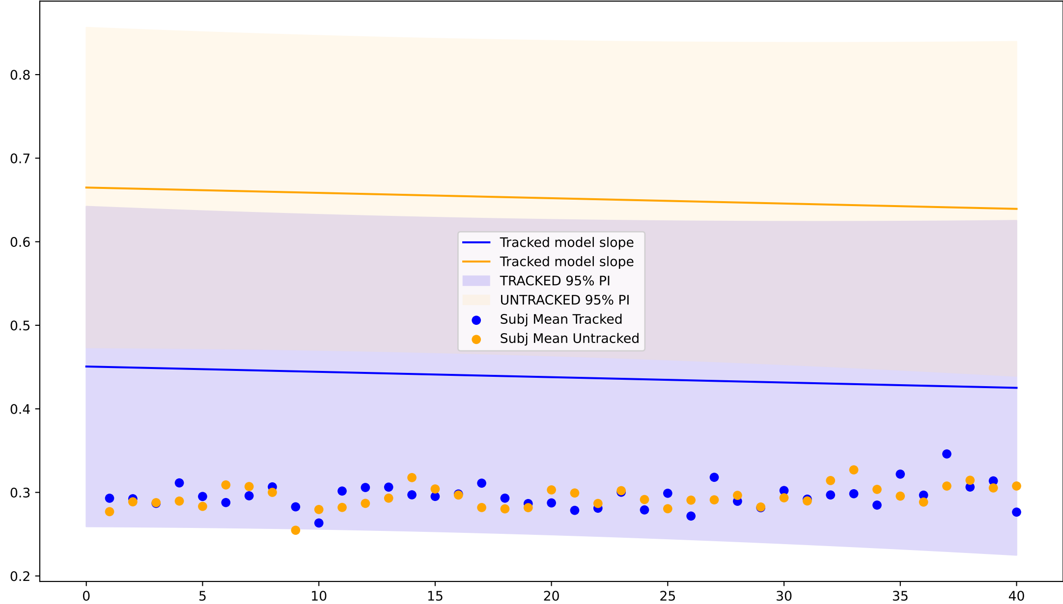
Lemma Embeddings FastText (Coef:0.2142 | P:0.5040)
