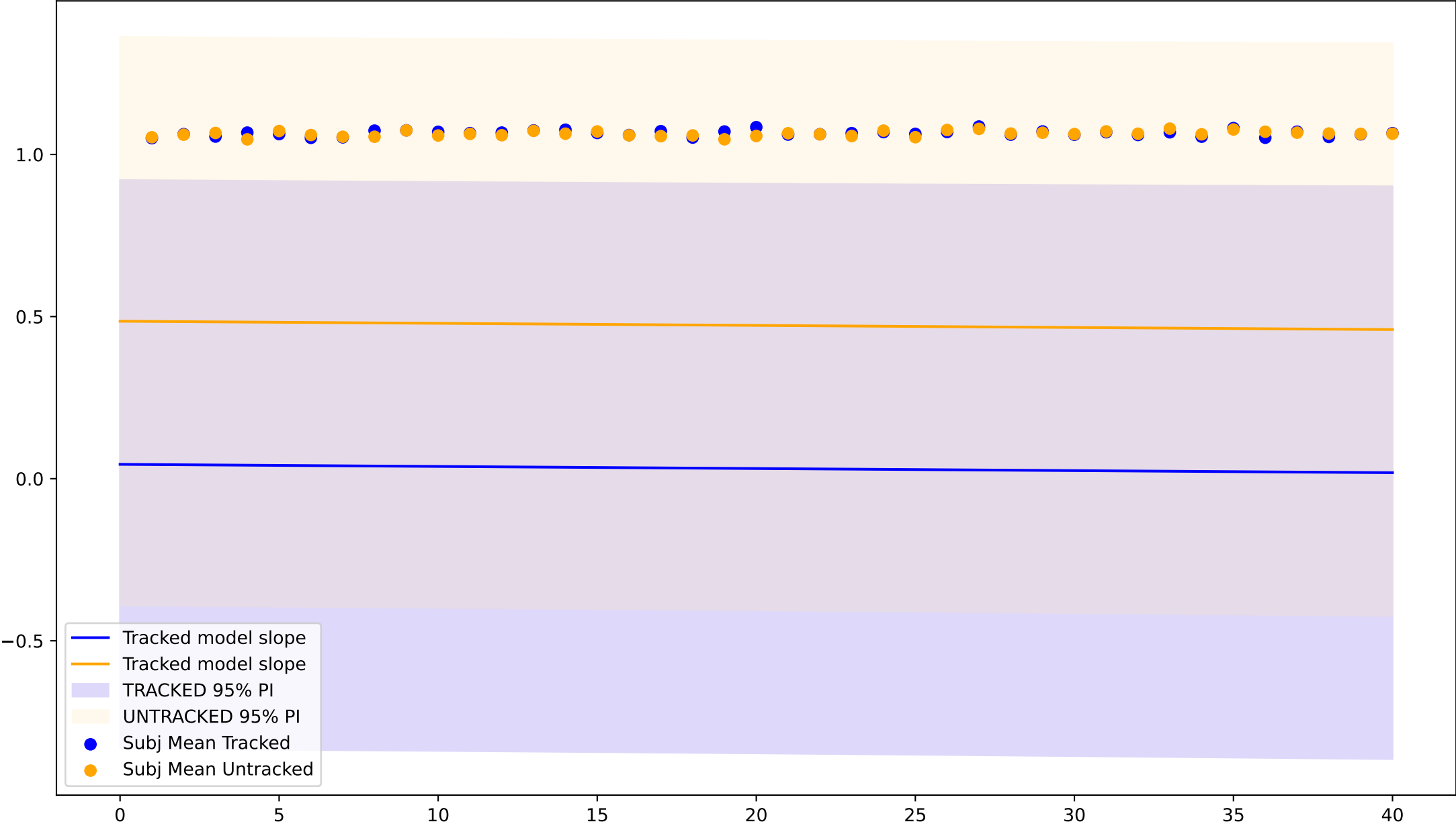
Word Mover Distance Subject (Coef:0.4414 | P:0.2935)
