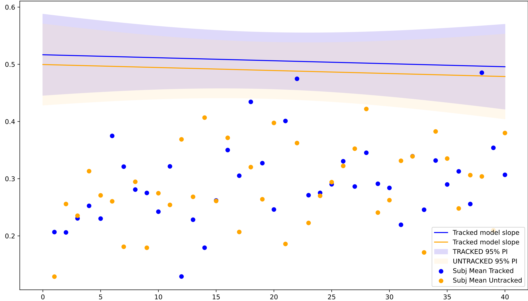
BERTopic TRT Prob (Coef:-0.0171 | P:0.7986)
