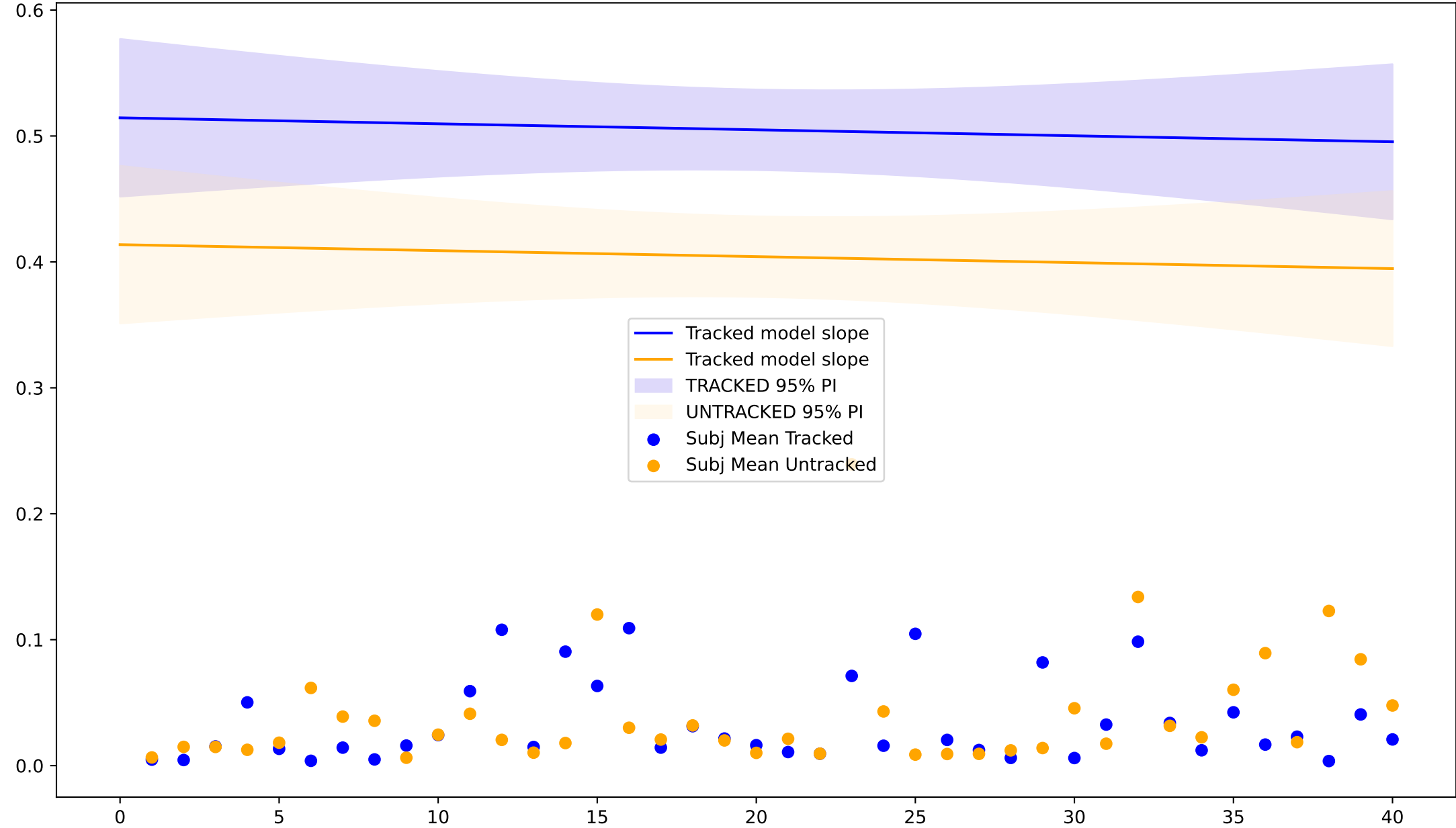
BERTopic MB Prob (Coef:-0.1007 | P:0.4219)
