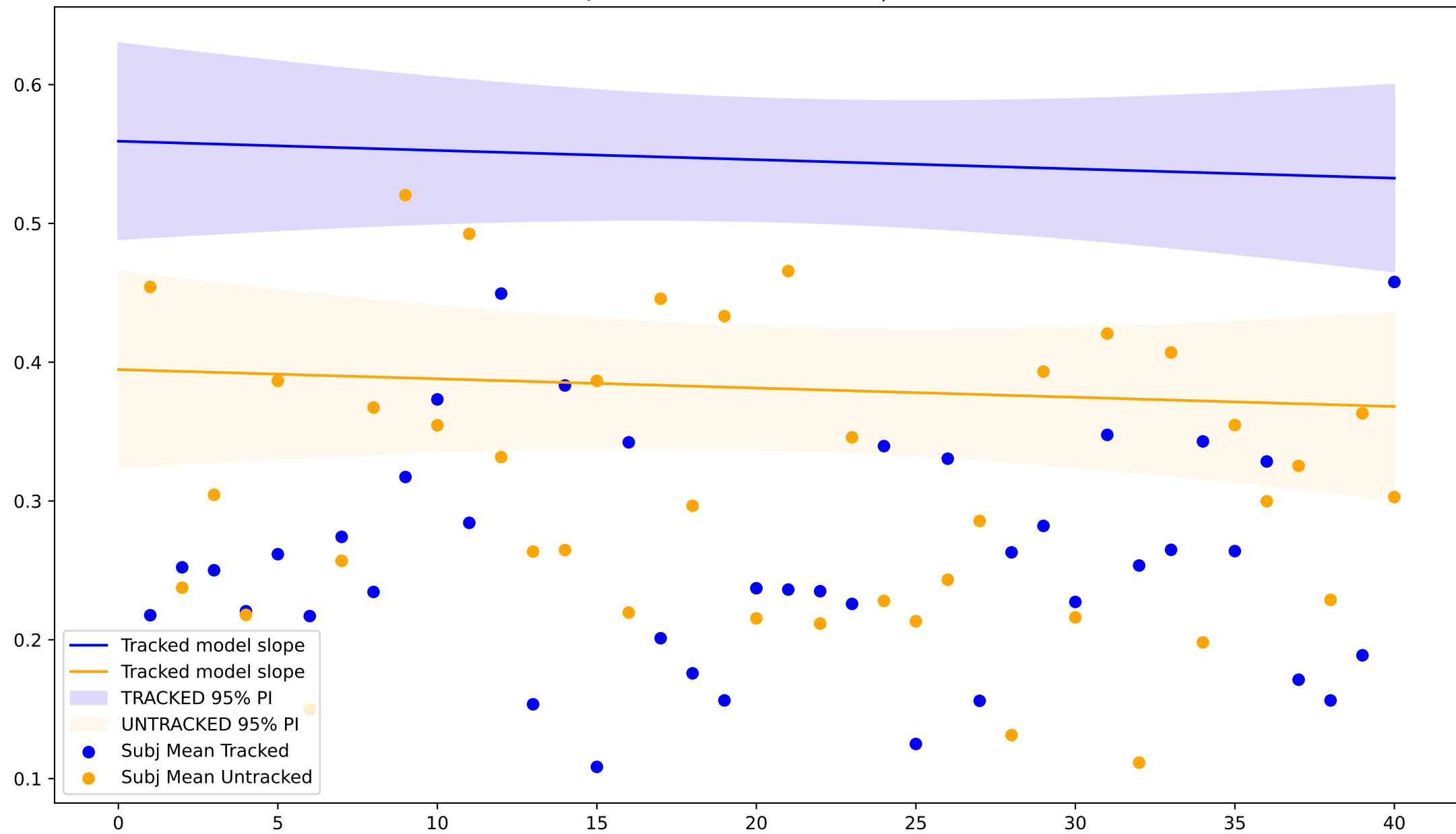
BERTopic MW Prob (Coef:-0.1645 | P:0.0062)
