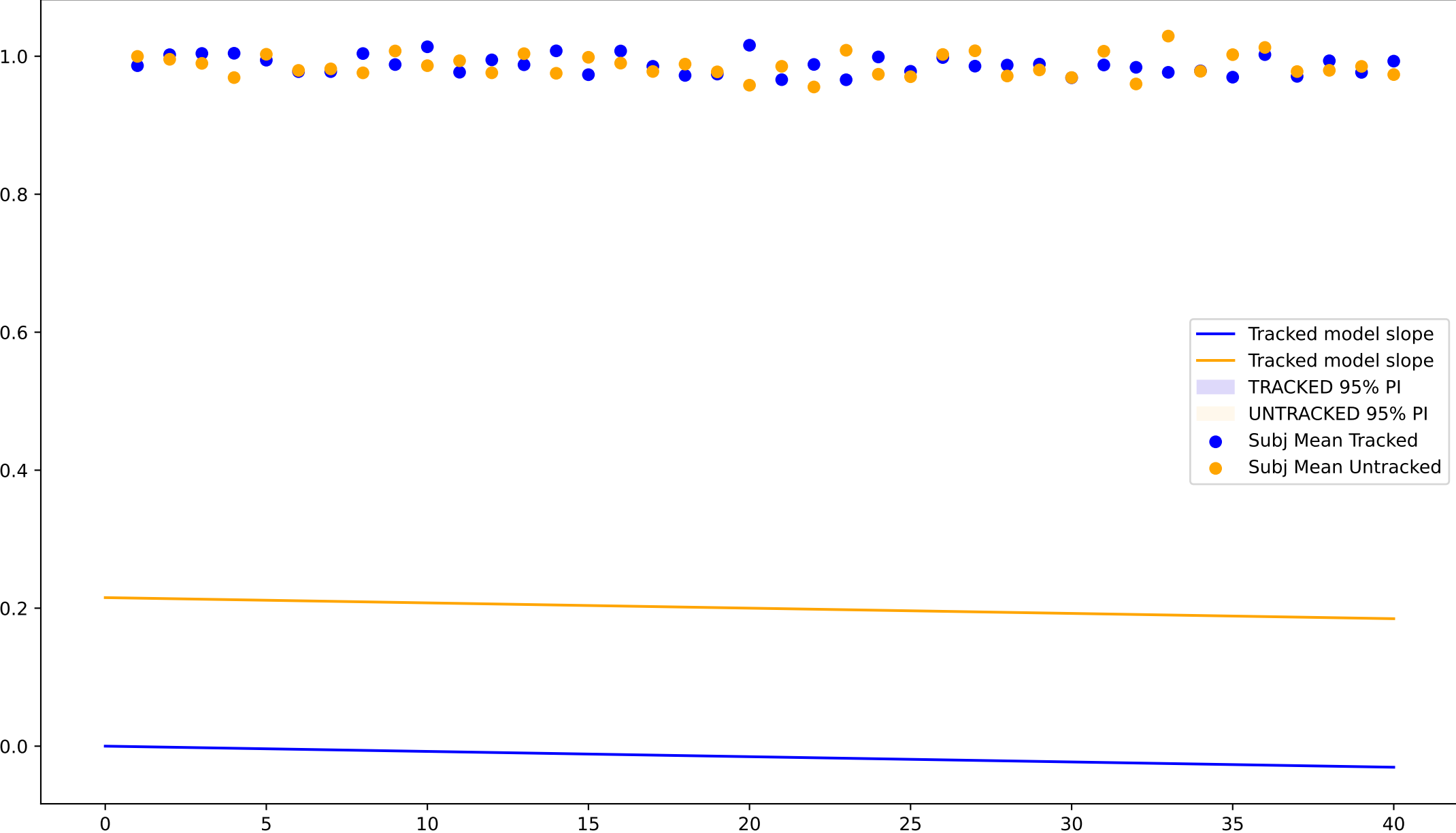
Word Mover Distance Dataset (Coef:0.2153 | P:0.5684)
