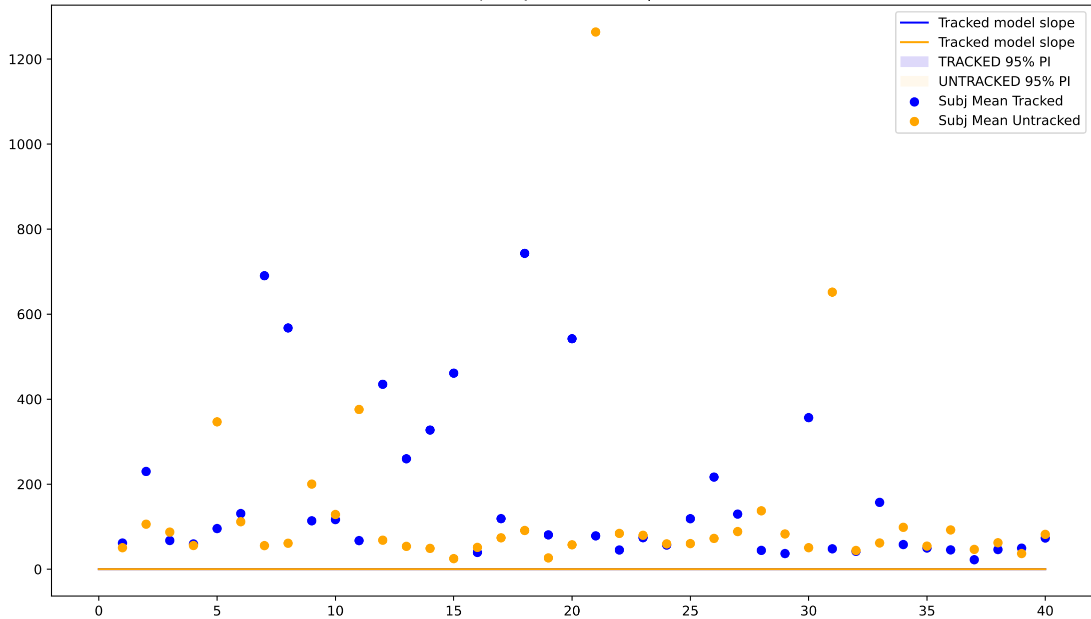
Bert Perplexity (Coef:0.0000 | P:0.3767)
