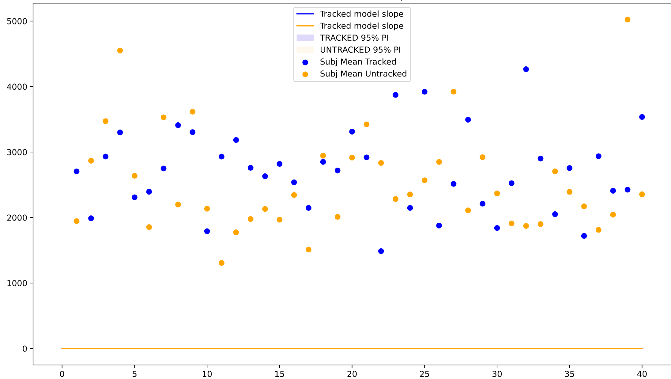
GLM Perplexity (Coef:0.0000 | P:0.2293)
