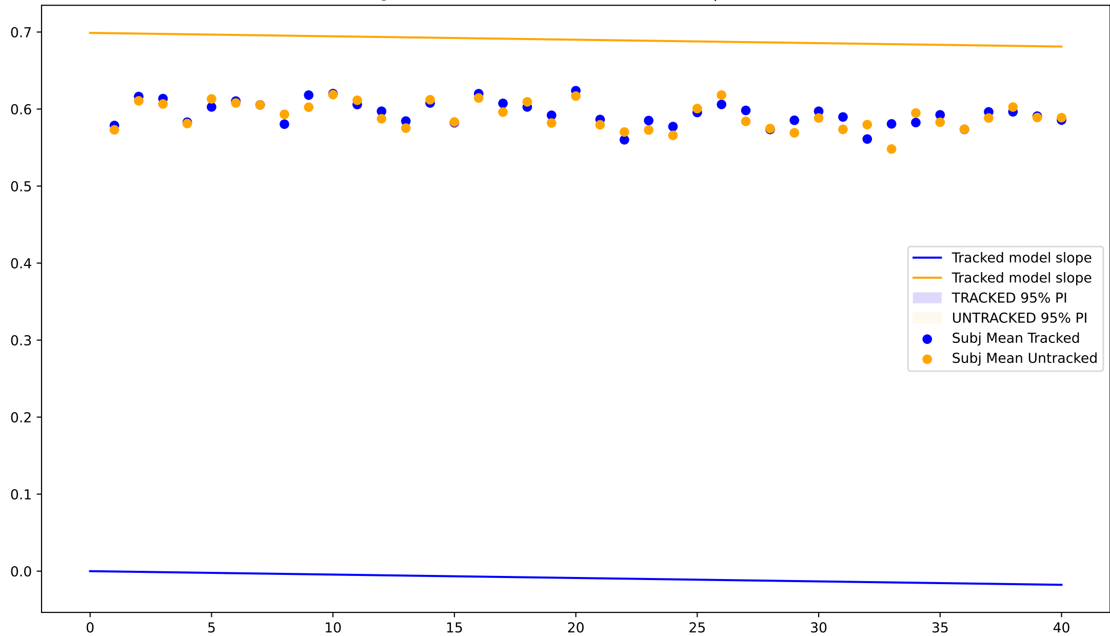
Frag-Utt Cosine Sim (Lemma) (Coef:0.6989 | P:0.2468)
