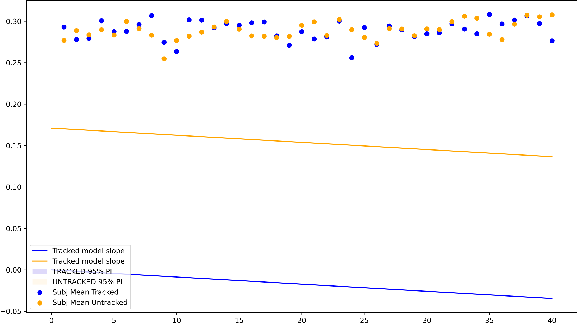
Lemma Embeddings FastText (Coef:0.1711 | P:0.7185)
