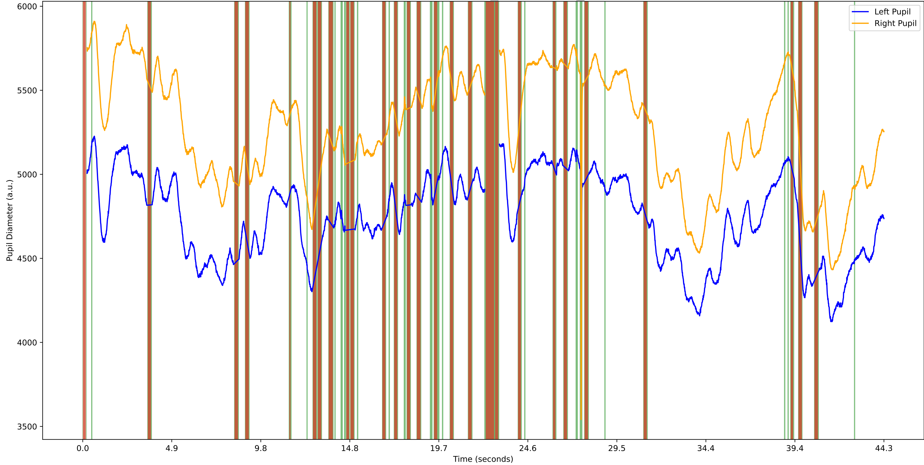
Interpolated Blinks: STORY_1 // JANEK_17 (13452.0)
