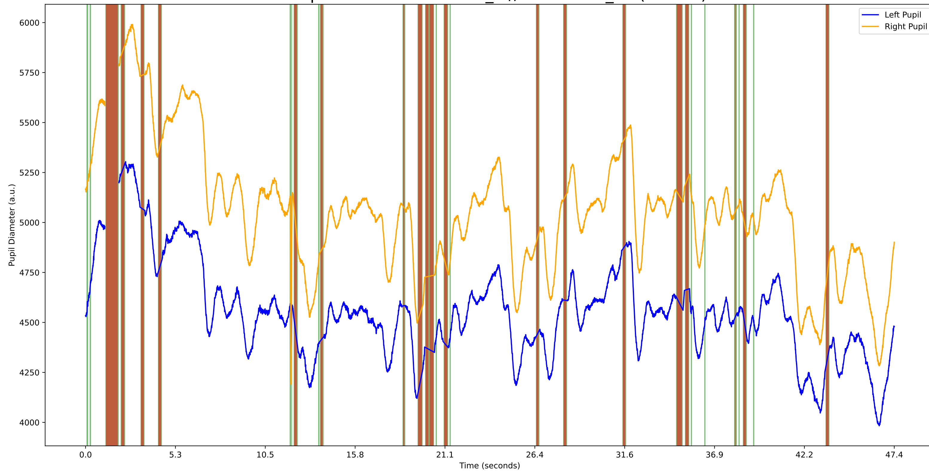
Interpolated Blinks: STORY_1 // KAROLINA_12 (9908.0)
