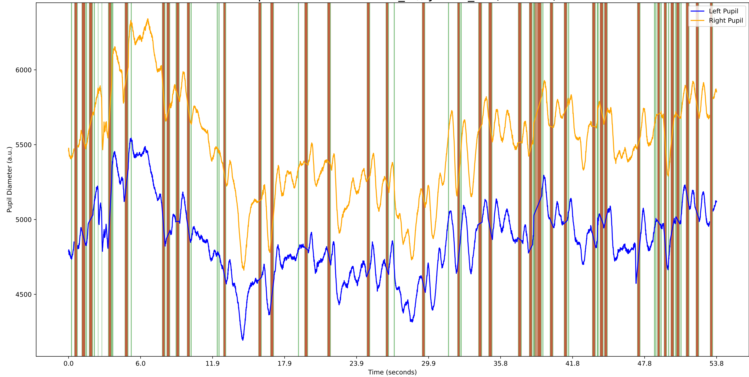
Interpolated Blinks: STORY_1 // JANEK_20 (21616.0)
