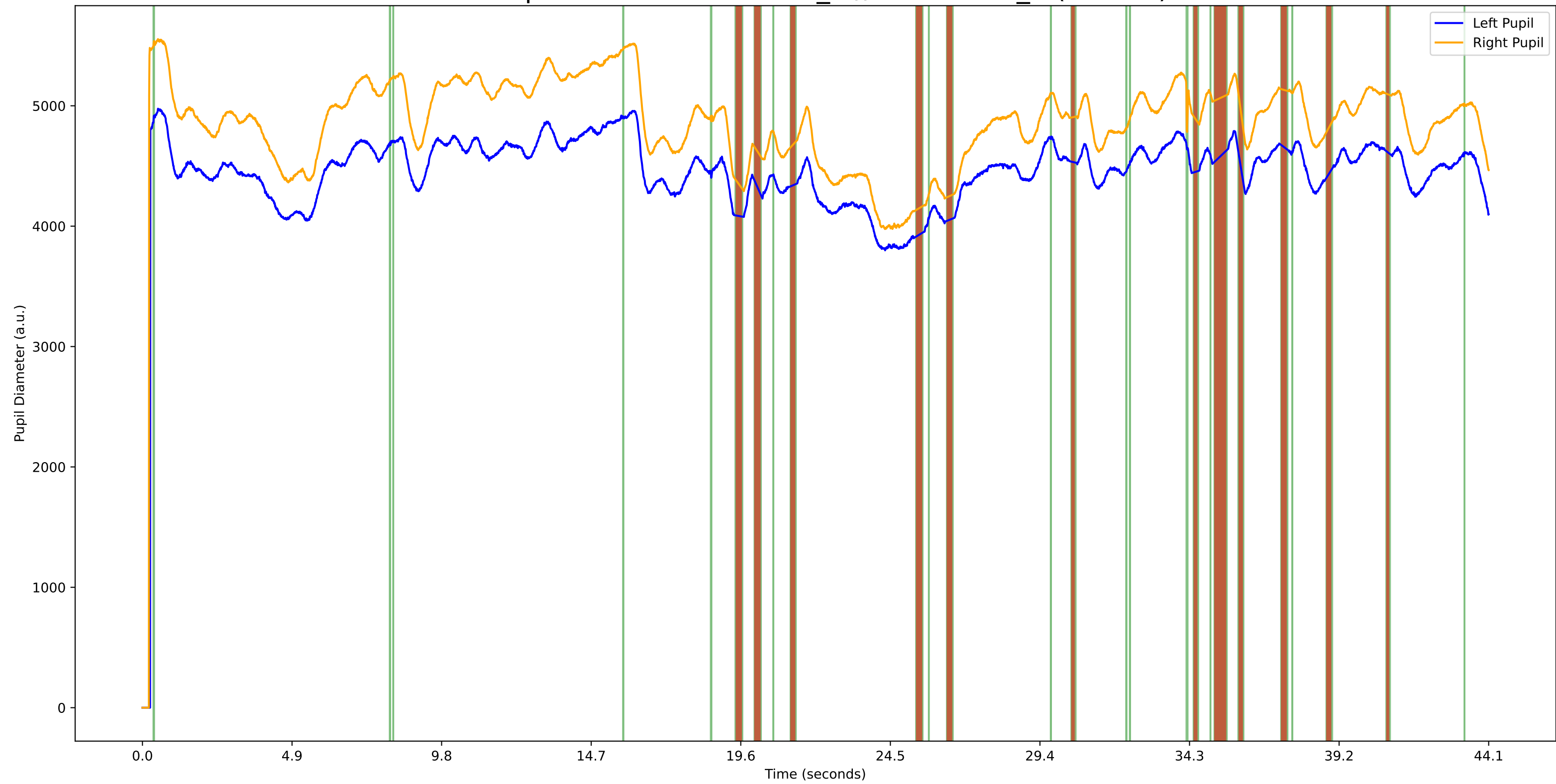
Interpolated Blinks: STORY_1 // KAROLINA_8 (7088.0)
