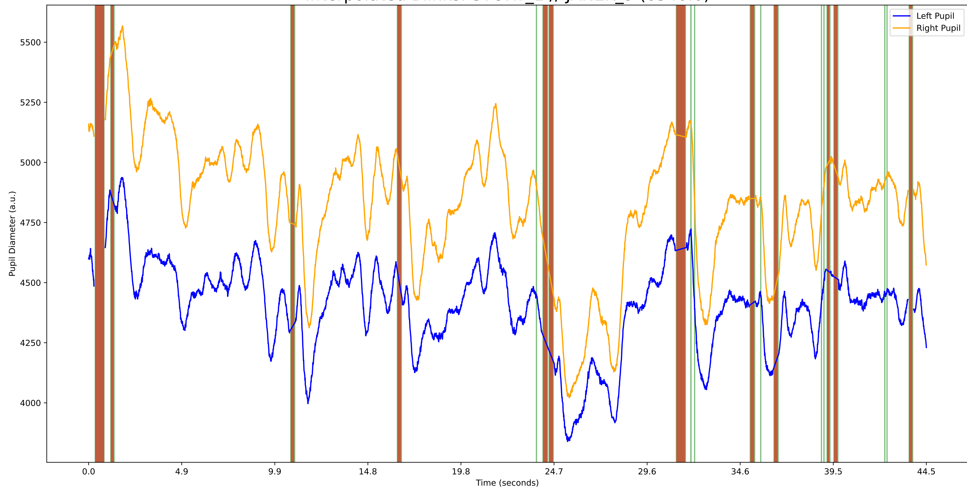
Interpolated Blinks: STORY_1 // JANEK_9 (6540.0)
