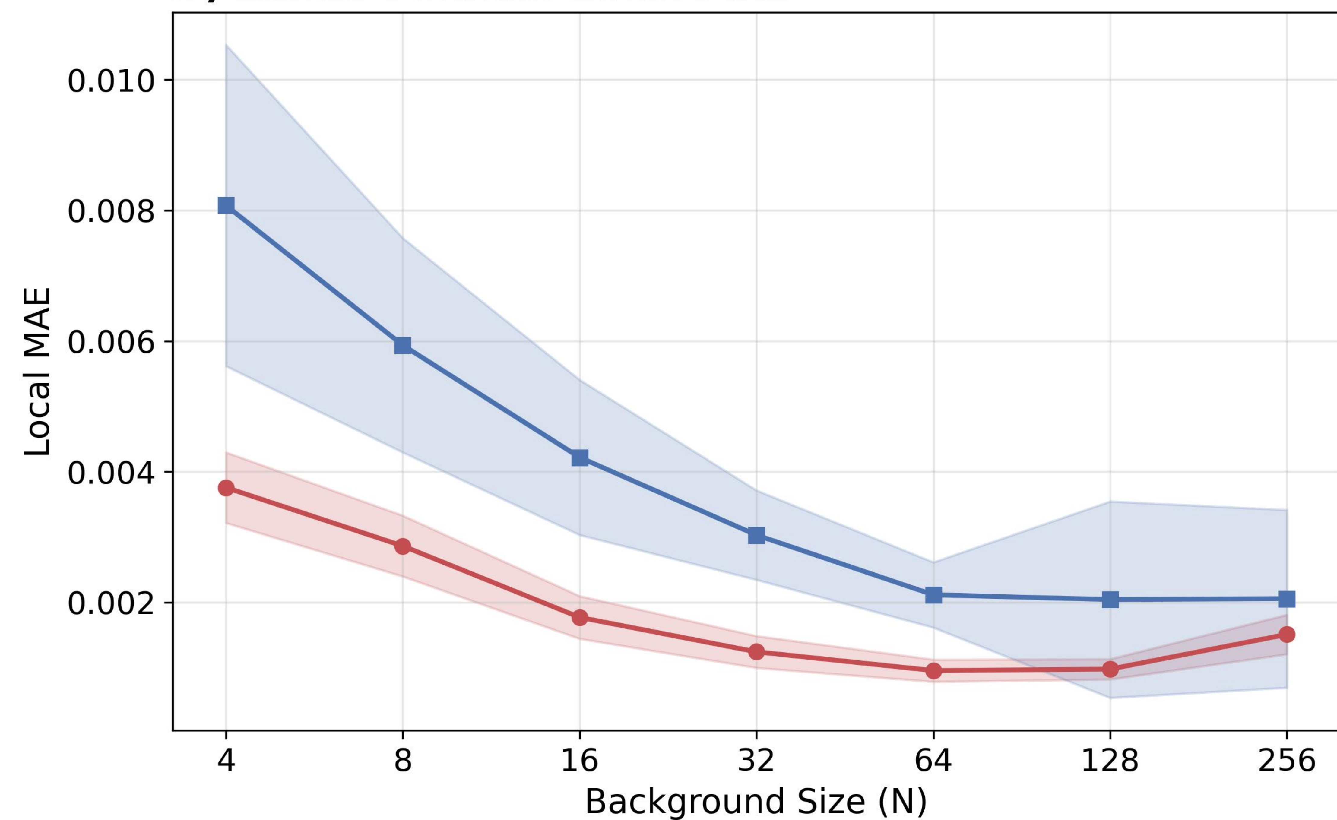
D) Linear Models: Local MAE
