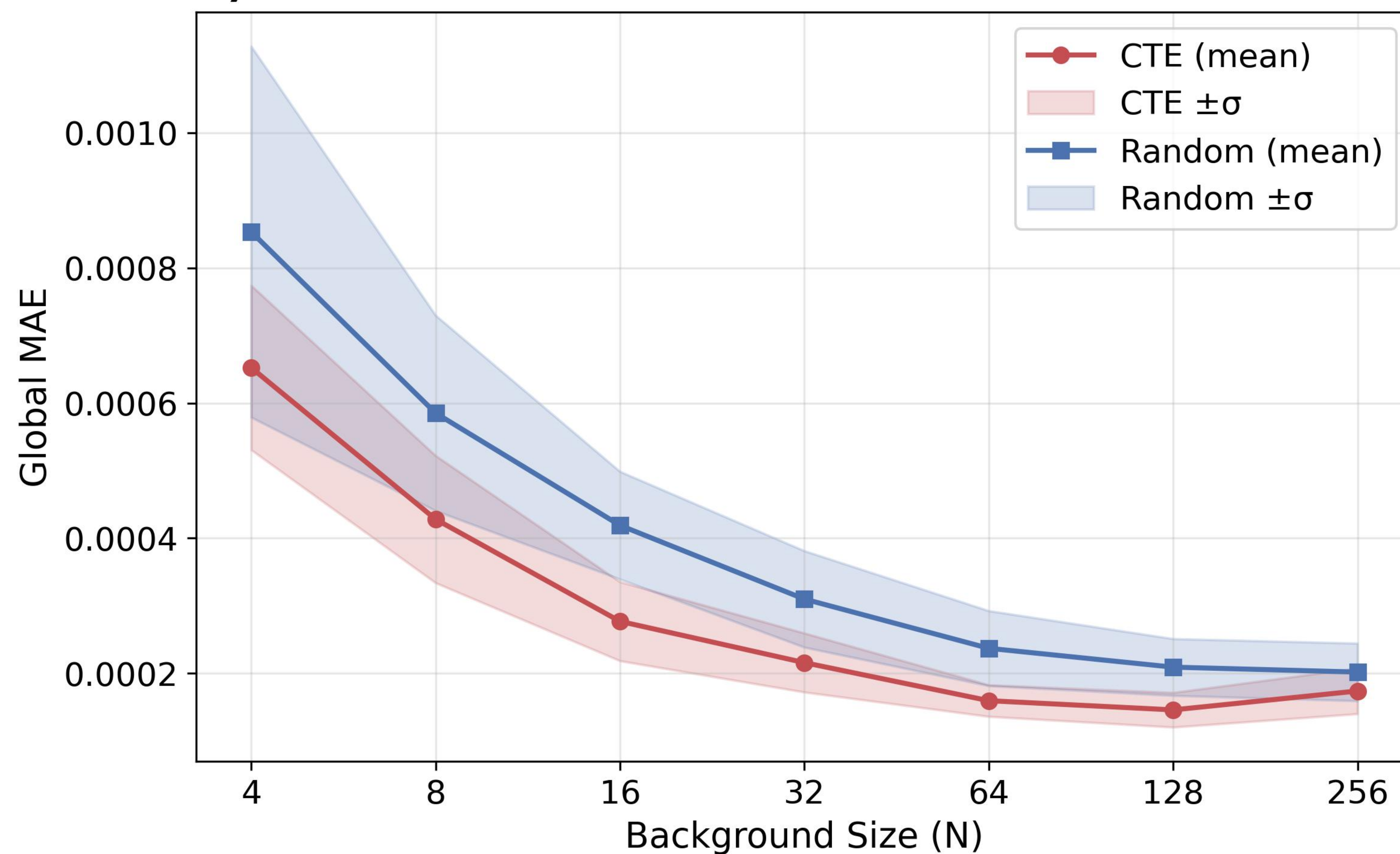
C) Linear Models: Global MAE
