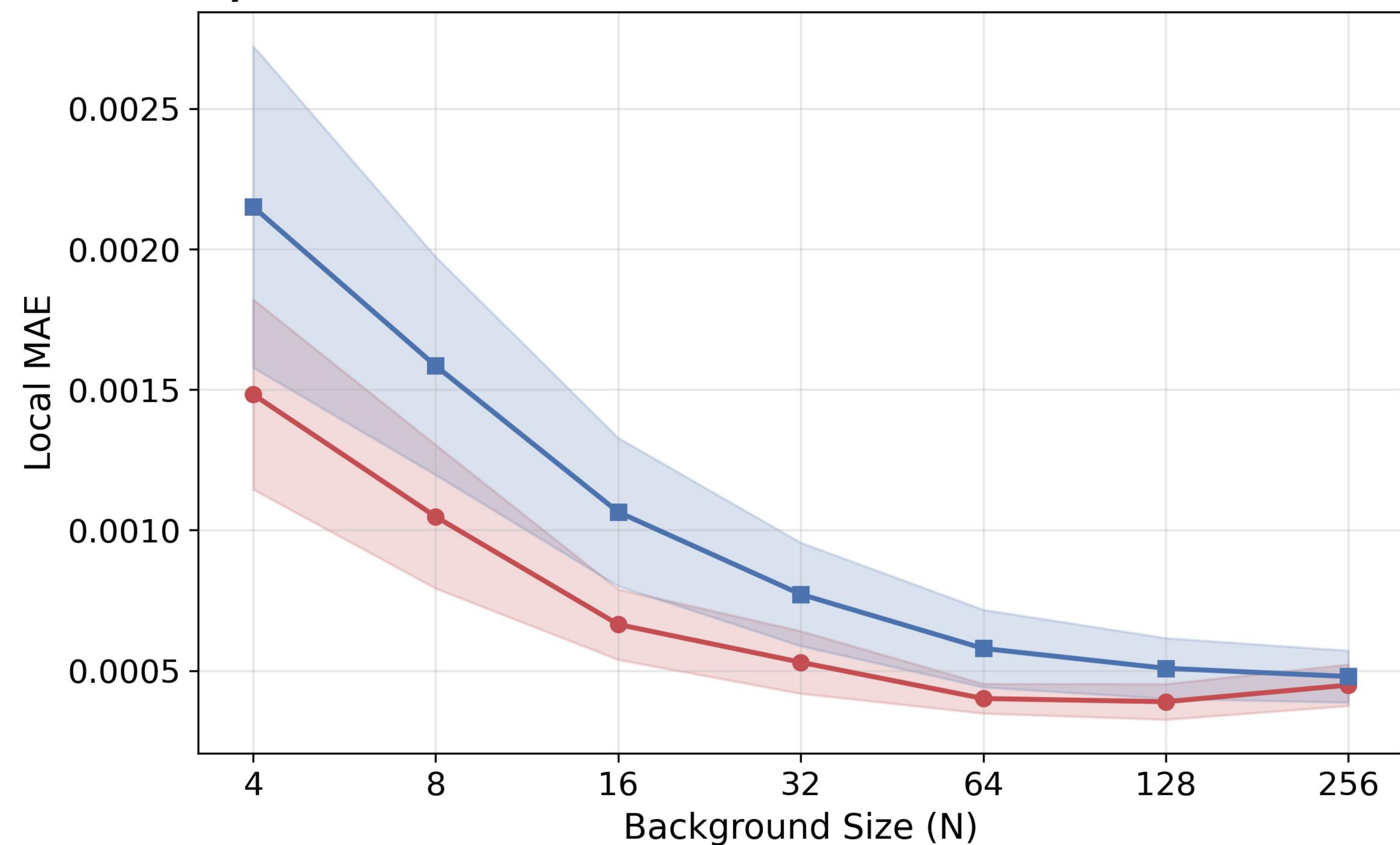
D) Linear Models: Local MAE
