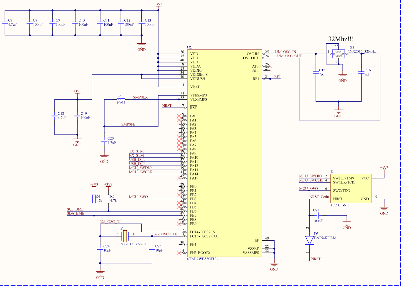
STM32 circuitry
