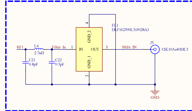
Bluetooth antenna circuitry
