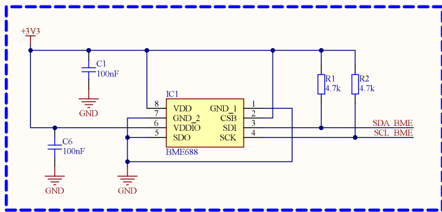
BME688 air quality sensor
