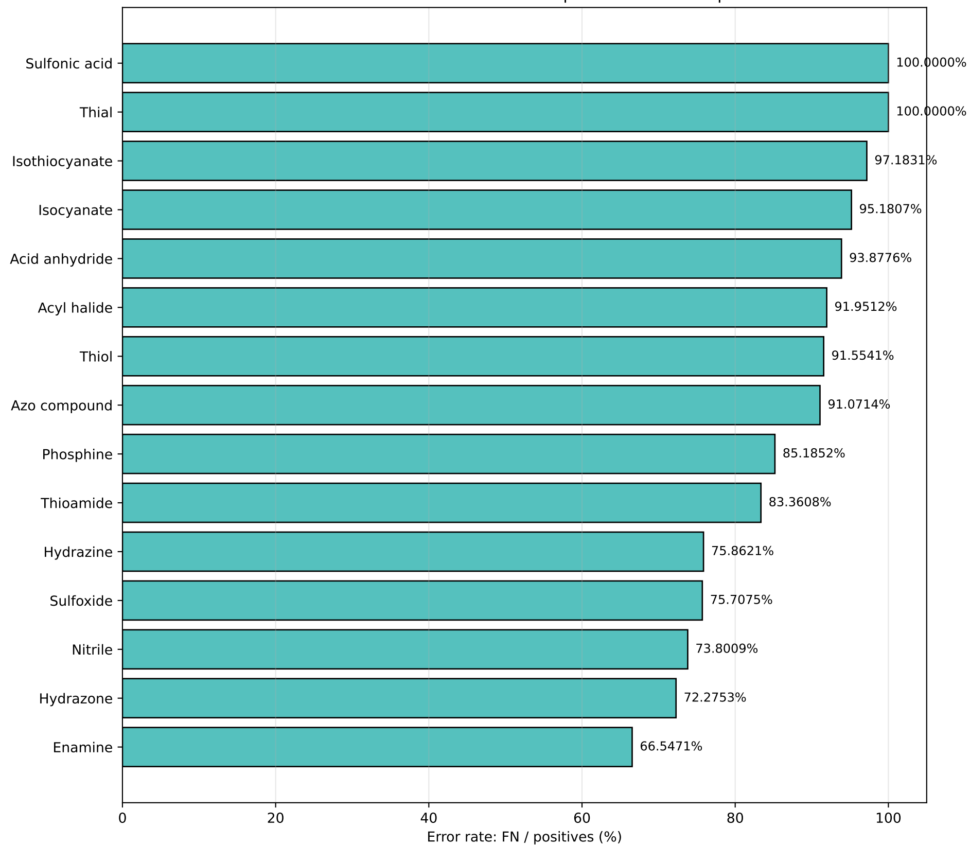
CNN H-NMR Validation Set - Top 15 Problem Groups
