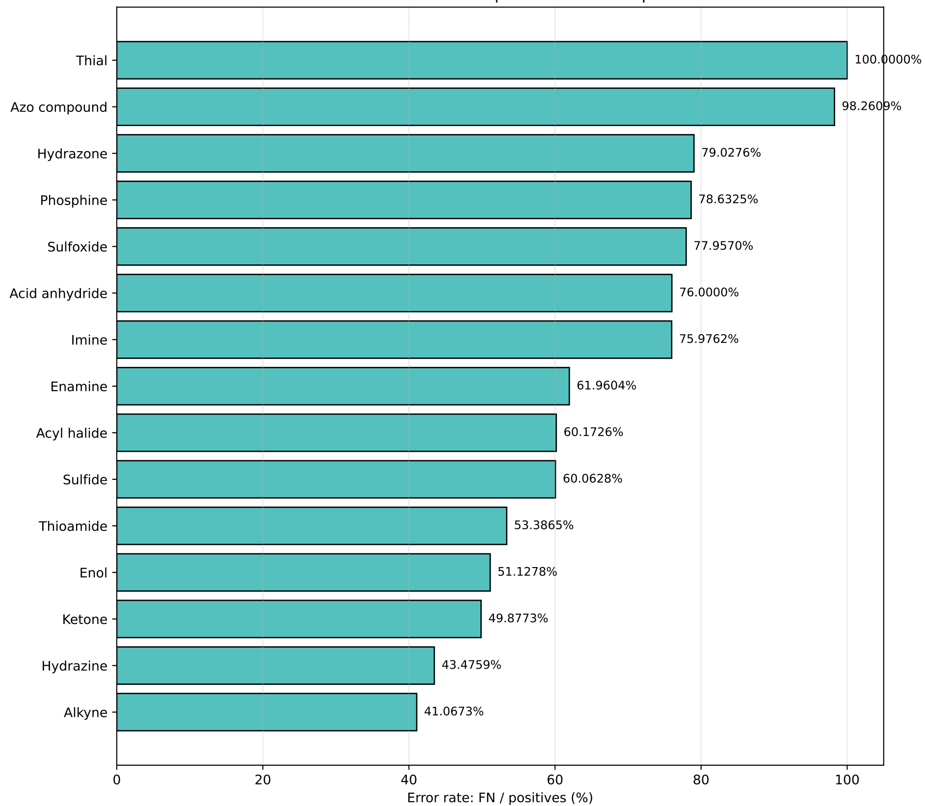
CNN IR Test Set - Top 15 Problem Groups
