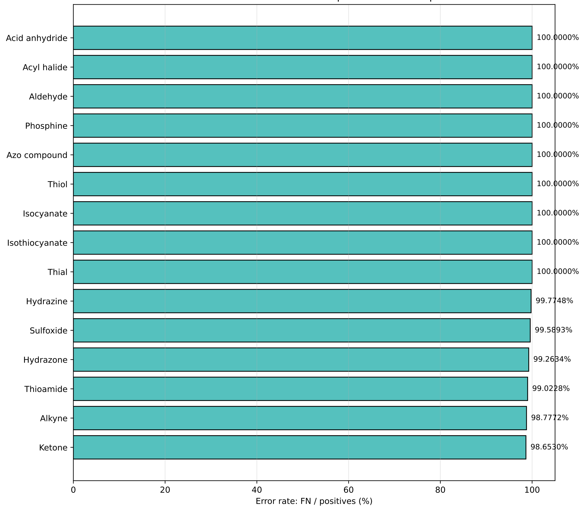
CNN MSMS- Validation Set - Top 15 Problem Groups
