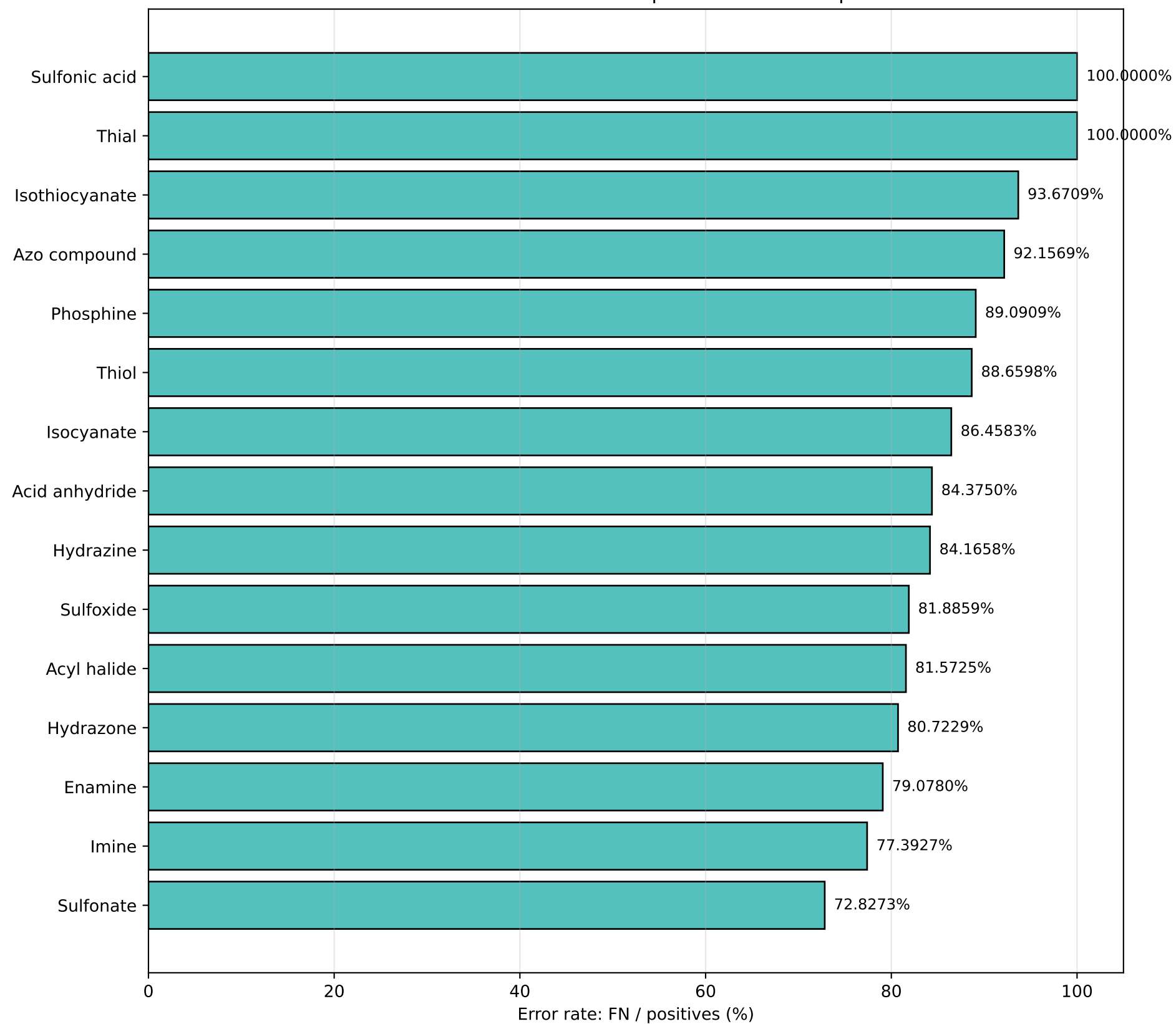
MPS C-NMR Test Set - Top 15 Problem Groups
