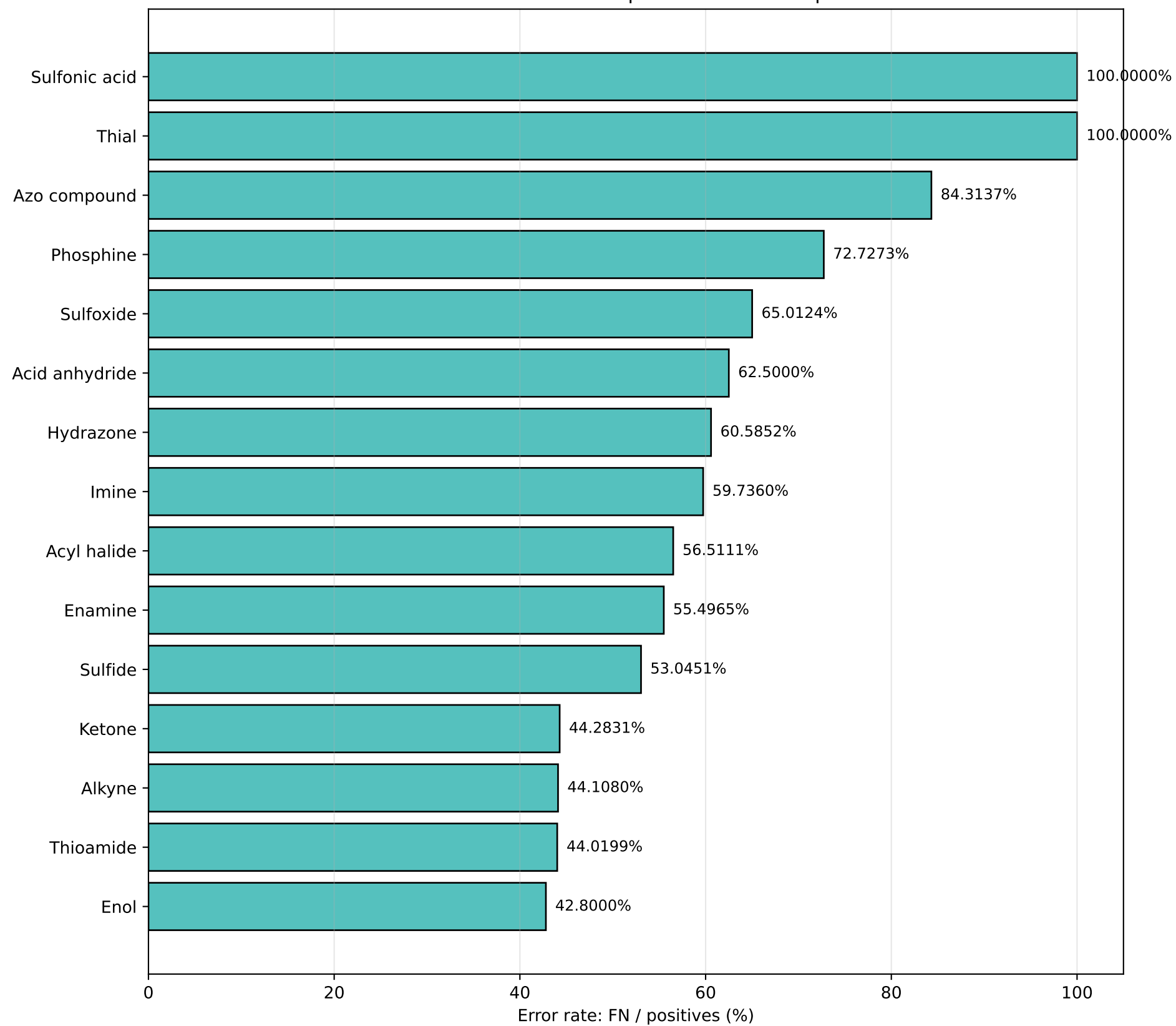
MPS IR Test Set - Top 15 Problem Groups
