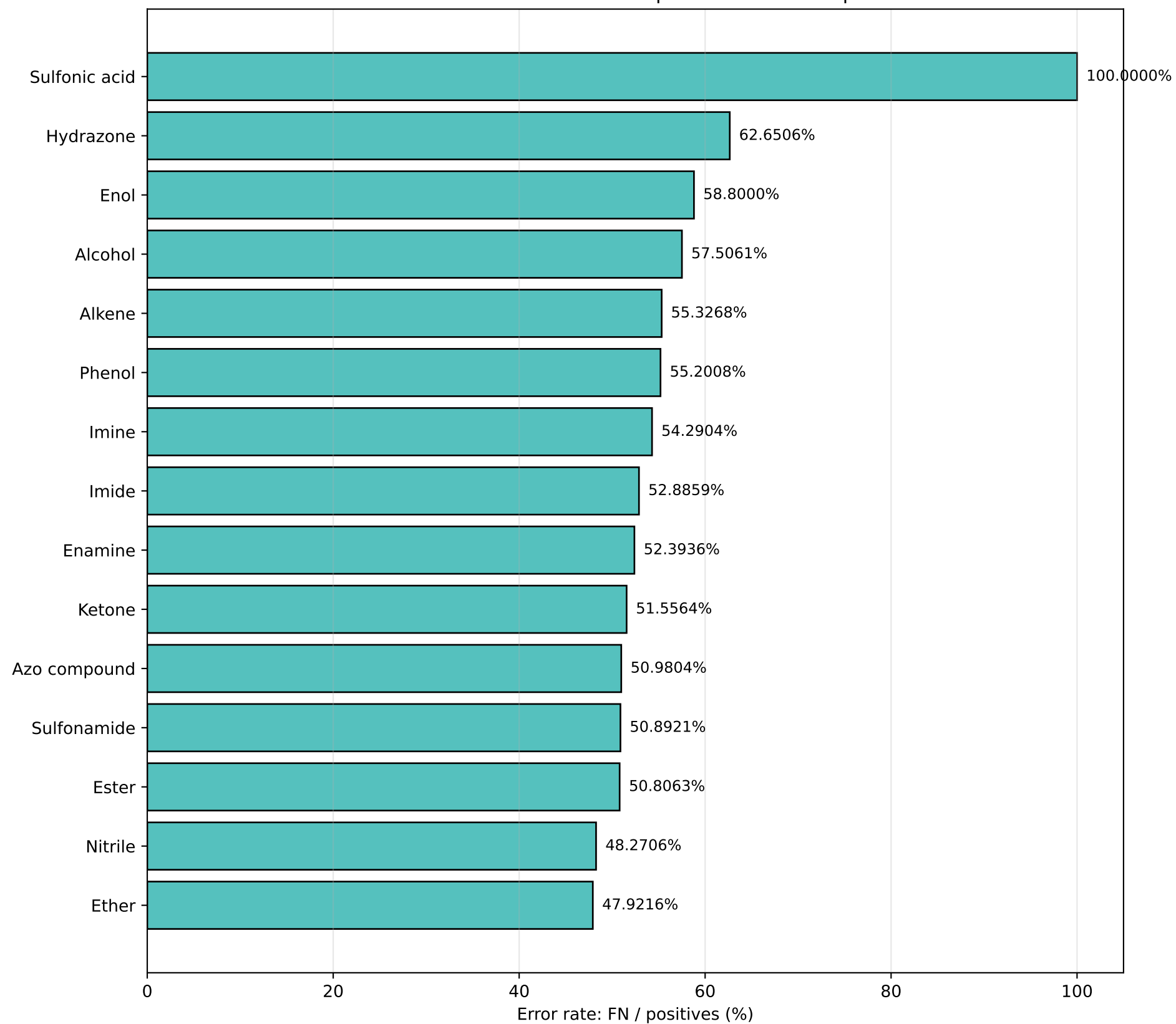
MPS MSMS+ Test Set - Top 15 Problem Groups
