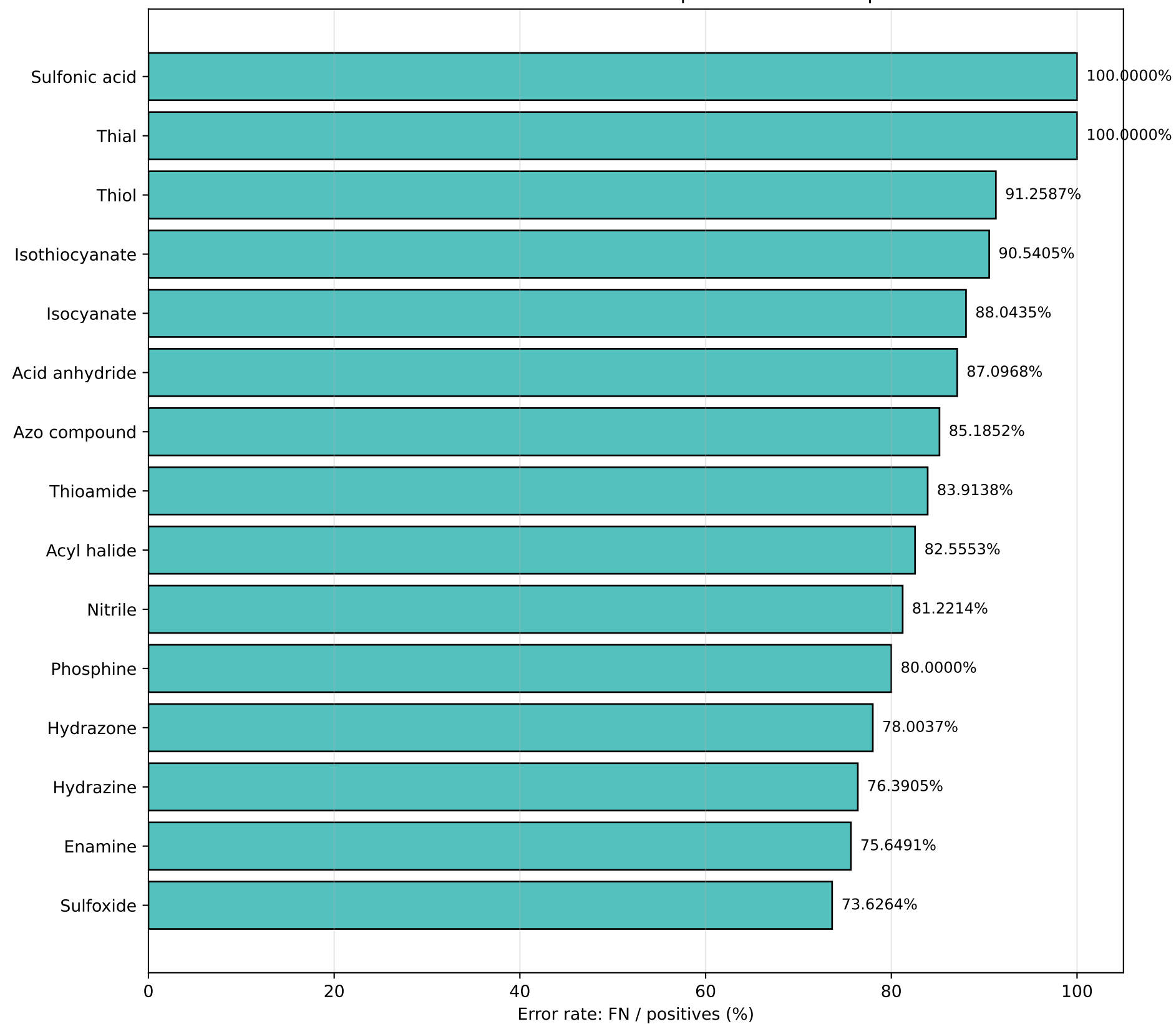
TTN H-NMR Validation Set - Top 15 Problem Groups
