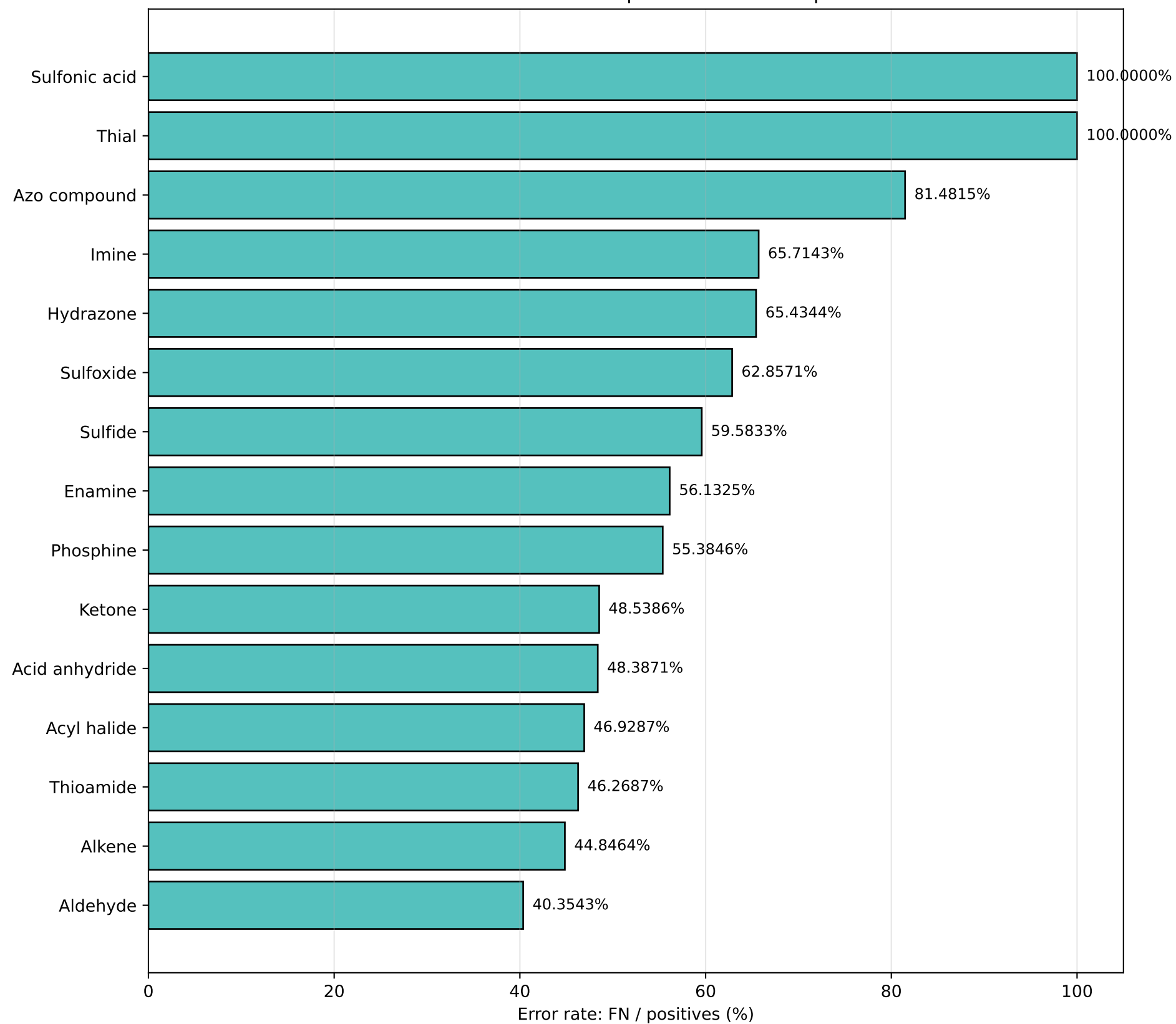
TTN IR Test Set - Top 15 Problem Groups
