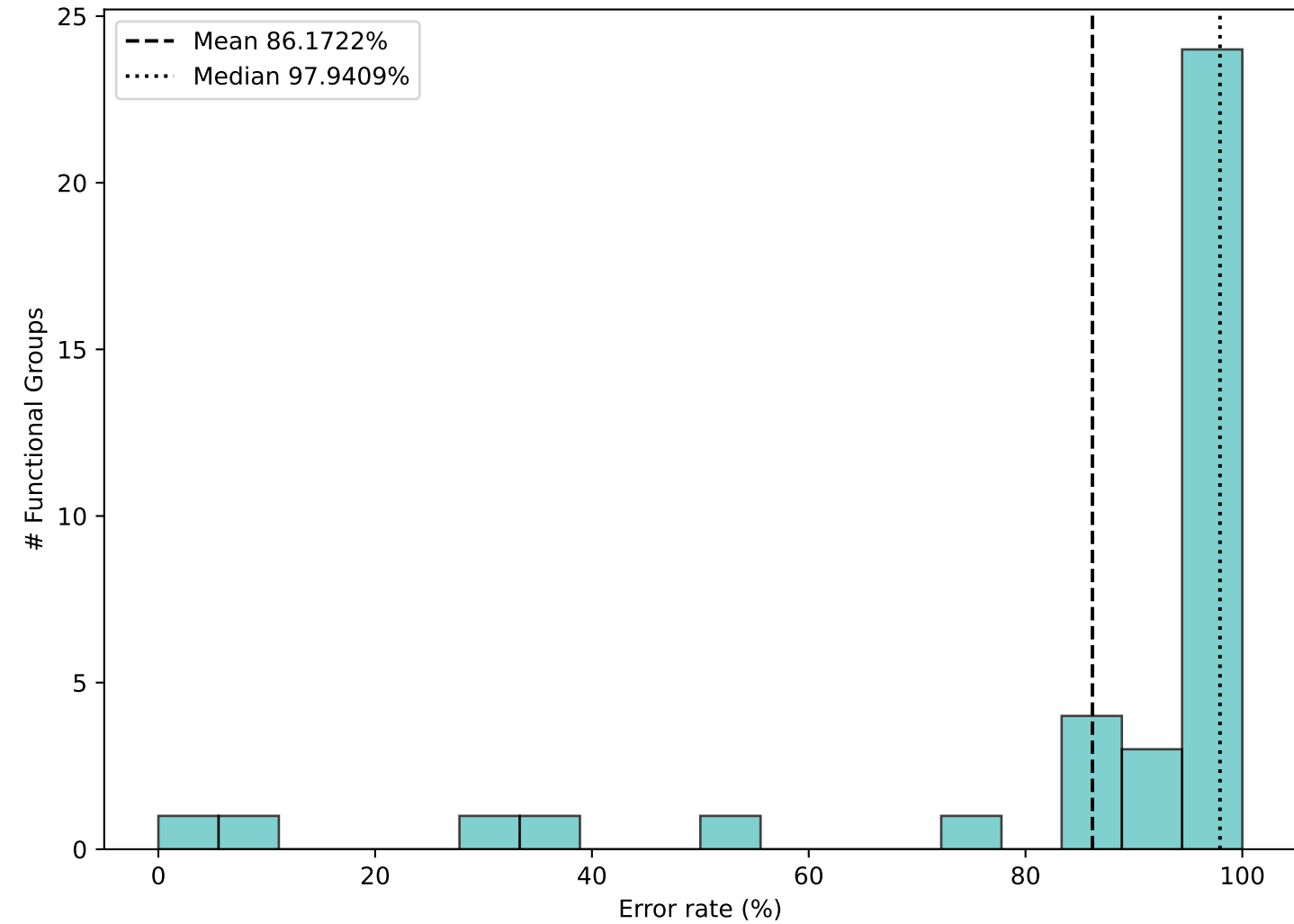
Error-Rate Distribution
