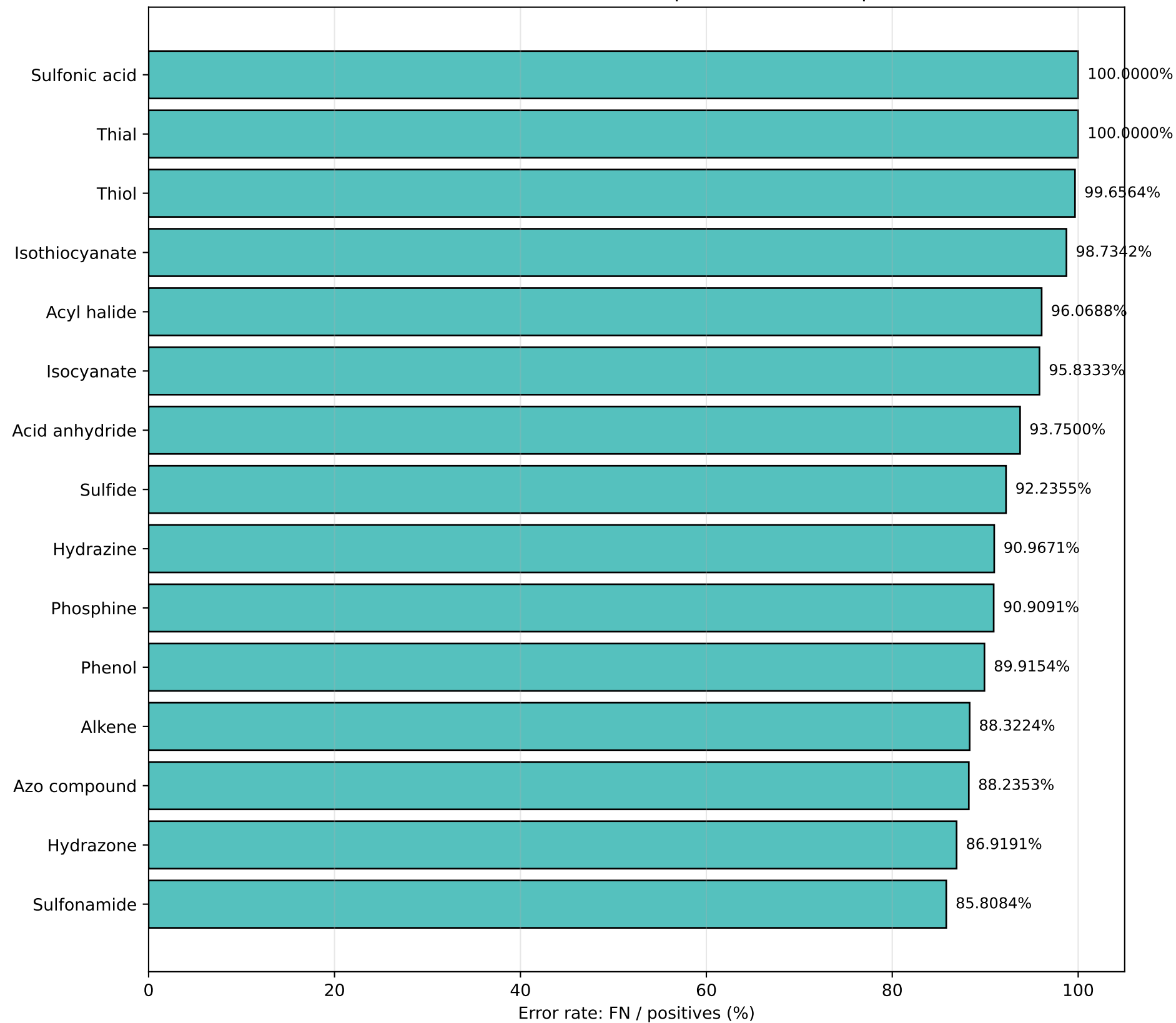
XGBoost C-NMR Test Set - Top 15 Problem Groups
