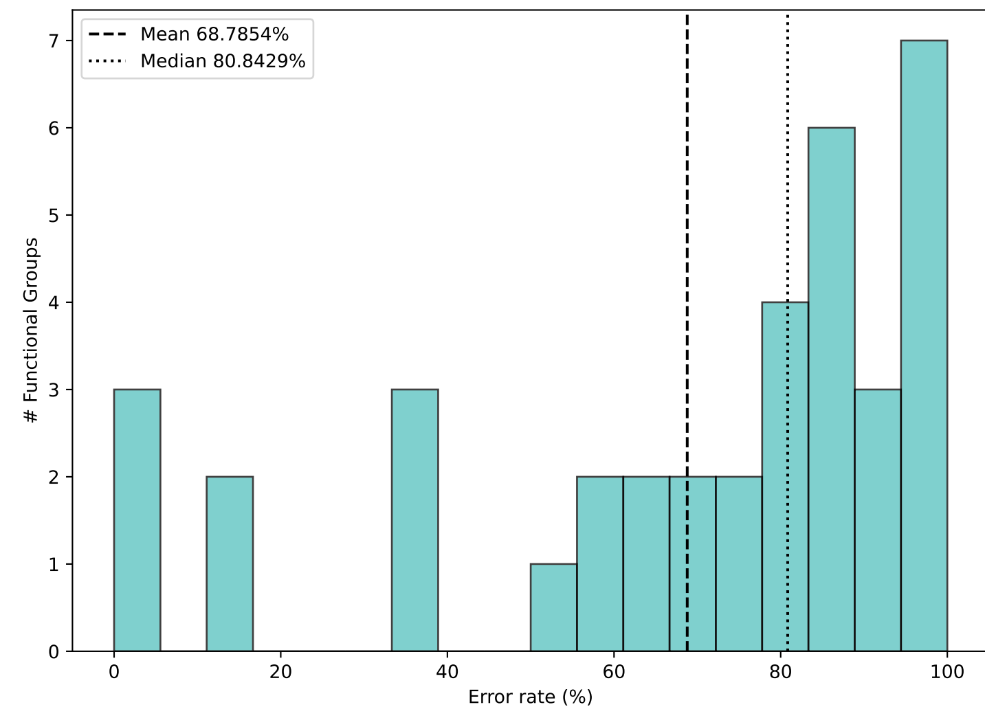
Error-Rate Distribution
