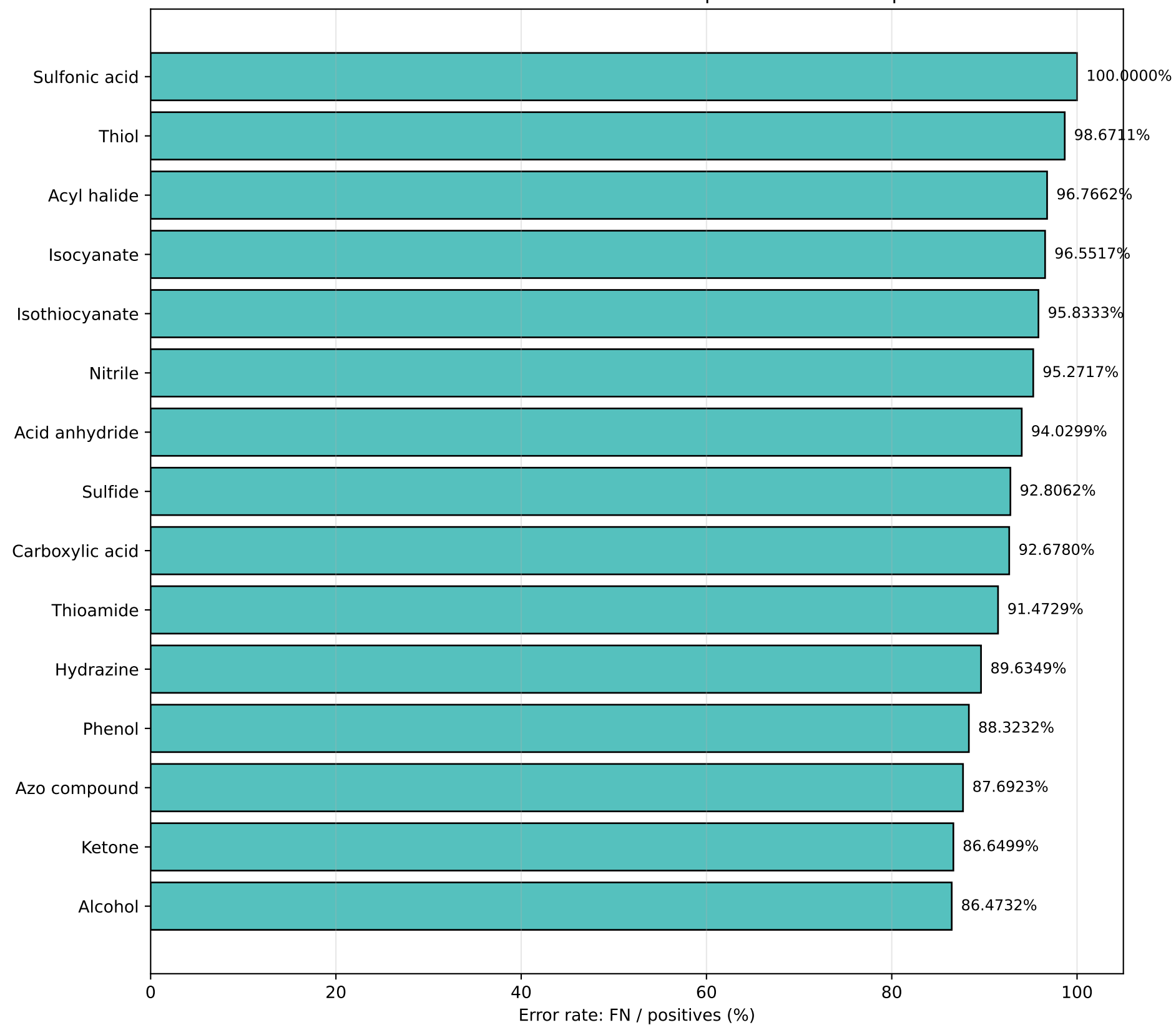
XGBoost H-NMR Validation Set - Top 15 Problem Groups
