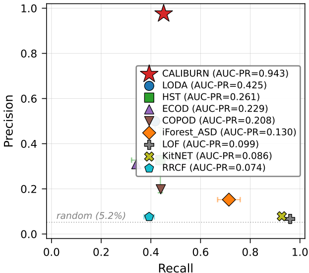
LITNET-2020: precision-recall operating points
