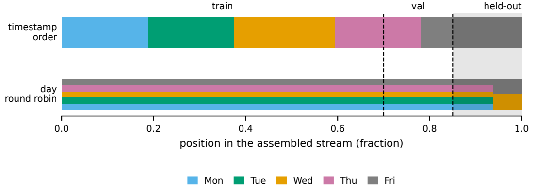
Figure 1: The two assemblies of the same CICIDS2017 records under one fixed positional split. In timestamp order the capture days follow one another, so the held-out slice is the tail of the last day. In day round robin every day still supplying records contributes to every position, so the held-out slice draws from the tail of each day. Block widths follow the per-day record budgets of Table 2. The figure is a schematic of the protocol and carries no measured value.
