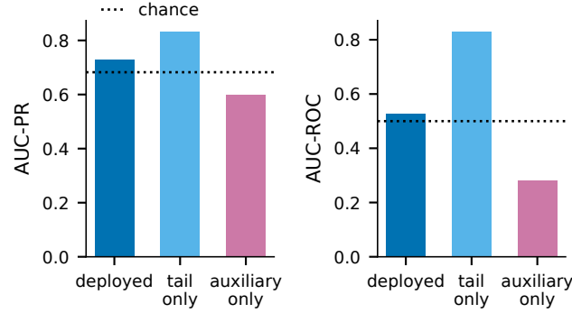
Fig. 4. Branch-wise discrimination on the timestamp-ordered held-out slice, the values of Table 6. Left: AUC-PR with the chance floor at the slice prevalence, 0.682350. Right: AUC-ROC with the chance level of an uninformative ranking. The deployed composition is the detector of the other figures. The tail term alone ranks above the deployed composition on both metrics, and the auxiliary term ranks below chance on AUC-ROC.
