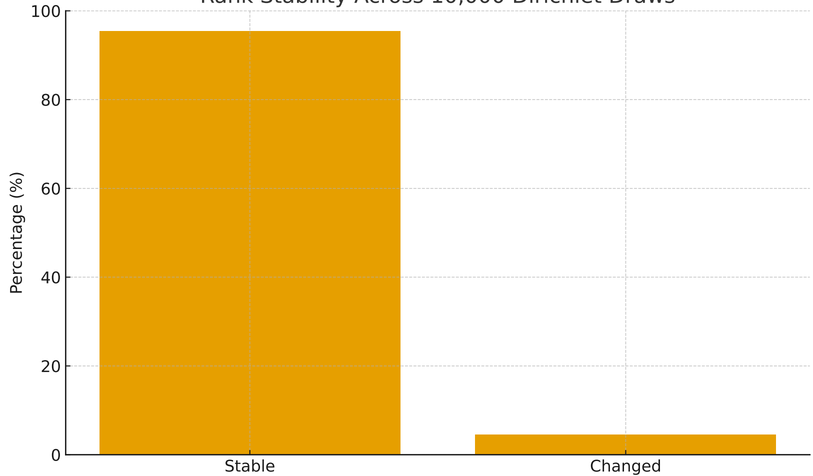
Rank Stability Across 10,000 Dirichlet Draws
