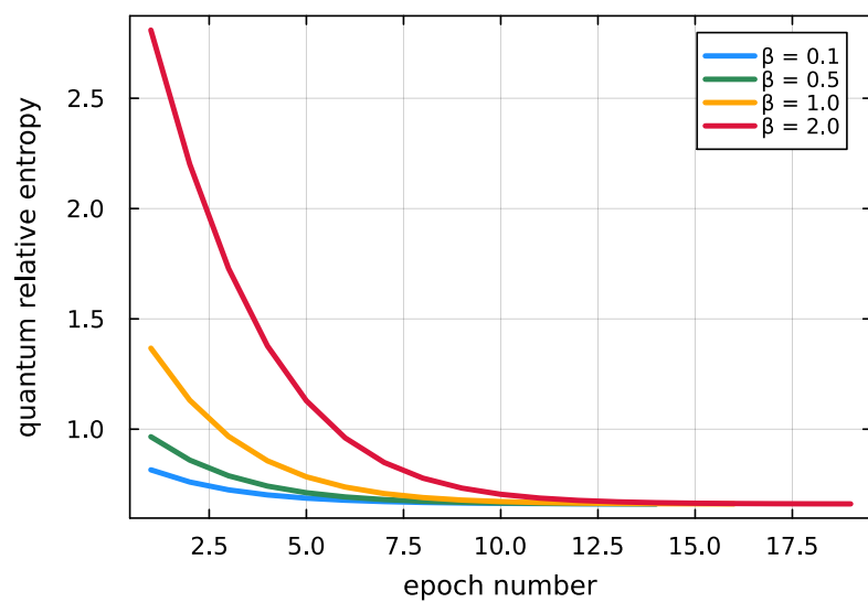
S(\eta || \rho_\theta) history
