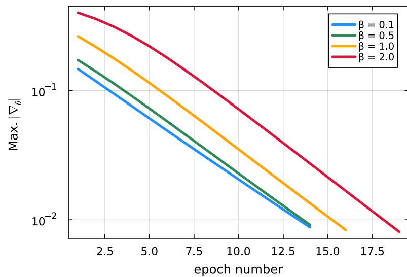
\max |\nabla_\theta| history
