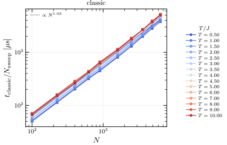
(c) Sweep time depending on the lattice size for all temperatures.
