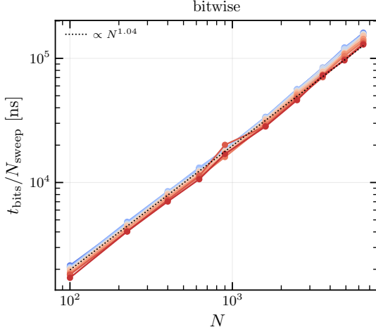
(c) Sweep time depending on the lattice size for all temperatures.
