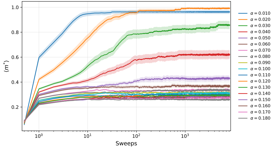
Figure 18: Evolution of \langle m^* \rangle with the storage load.
