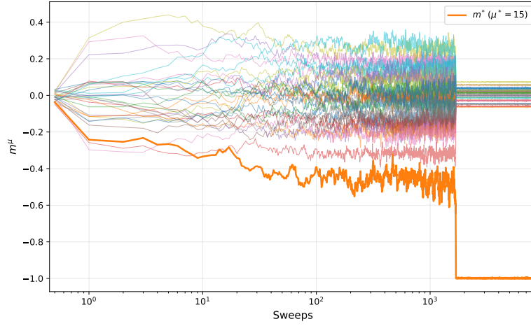
Figure 16: Evolution of m^\mu for all patterns for the replica 16 of \alpha = 0.03 .
