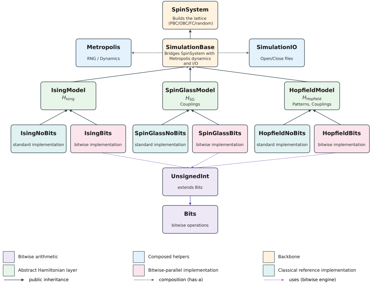
Figure 6: Code structure
