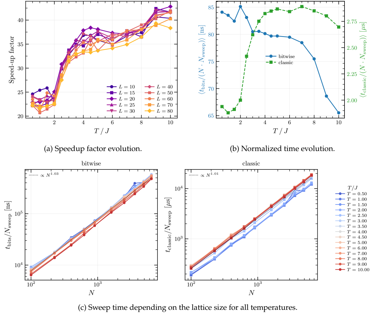
Figure 10: Performance analysis of the bitwise and classical Ising Metropolis implementations. Subfigure (a) shows the evolution of the speedup factor with the temperature for several size of square lattices. (b) shows the evolution of the normalized spin update time with the temperature, averaged over the different lattice sizes. Finally, (c) presents the evolution of the time taken to perform one sweep with the lattice size for different temperatures.
