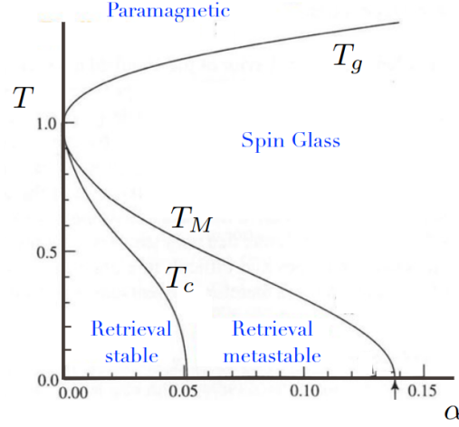
Figure 13: Phase diagram of the Hopfield model in the thermodynamic limit ( N \rightarrow \infty ), extracted from [19]. the phase transition value at T = 0 is signified by the arrow.
