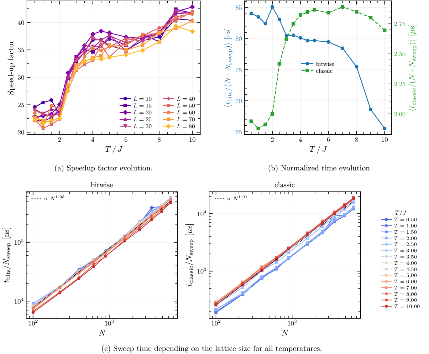
Figure 5: Performance analysis of the bitwise and classical Ising Metropolis implementations. Subfigure (a) shows the evolution of the speedup factor with the temperature for several sizes of square lattices. (b) shows the evolution of the normalized spin update time with the temperature, averaged over the different lattice sizes. Finally, (c) presents the evolution of the time taken to perform one sweep depending on the lattice size, for different temperatures.
