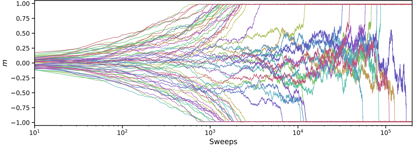
Figure 3: Trajectories of the 64 magnetizations over time for L = 100 and T/J = 1.5 . All those trajectories have been obtained from the same simulation. While some realizations quickly collapse into the equilibrium attractors m_{\pm} = \pm 0.953 , some require \sim 10^2 times more sweeps to reach the same equilibrium.
