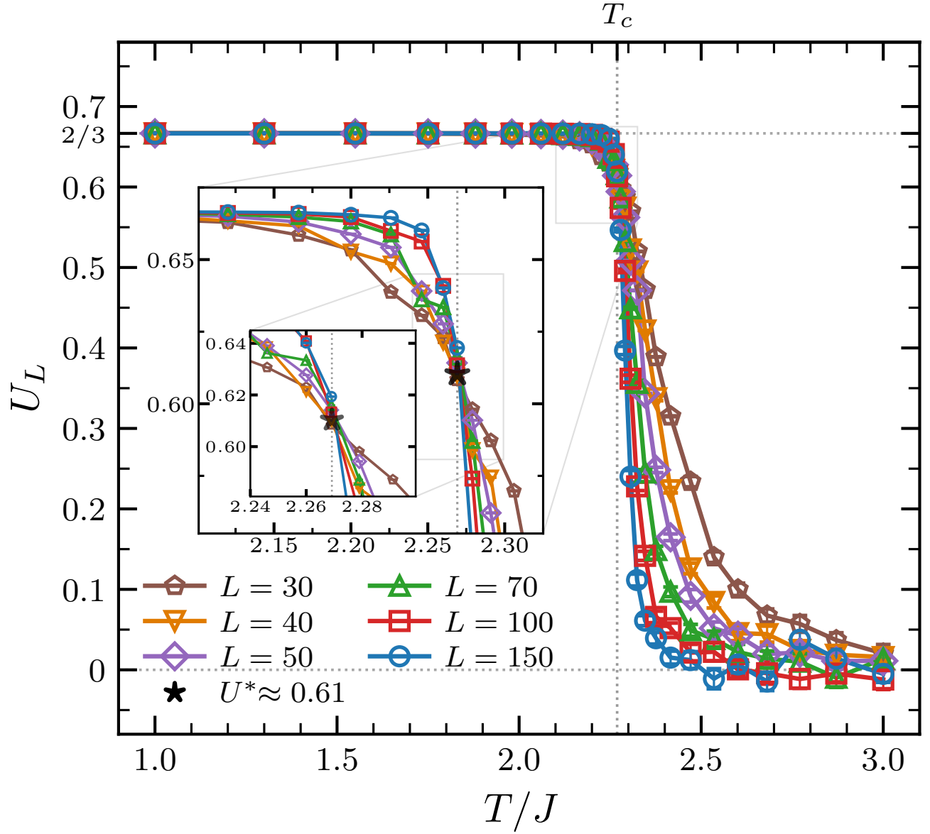
Figure 4: Binder cumulant for the different lattice sizes. The curves approach the two asymptotic limits and intersect at (T_c, U^*) , as expected. Insets show the zoomed region around the critical point.
