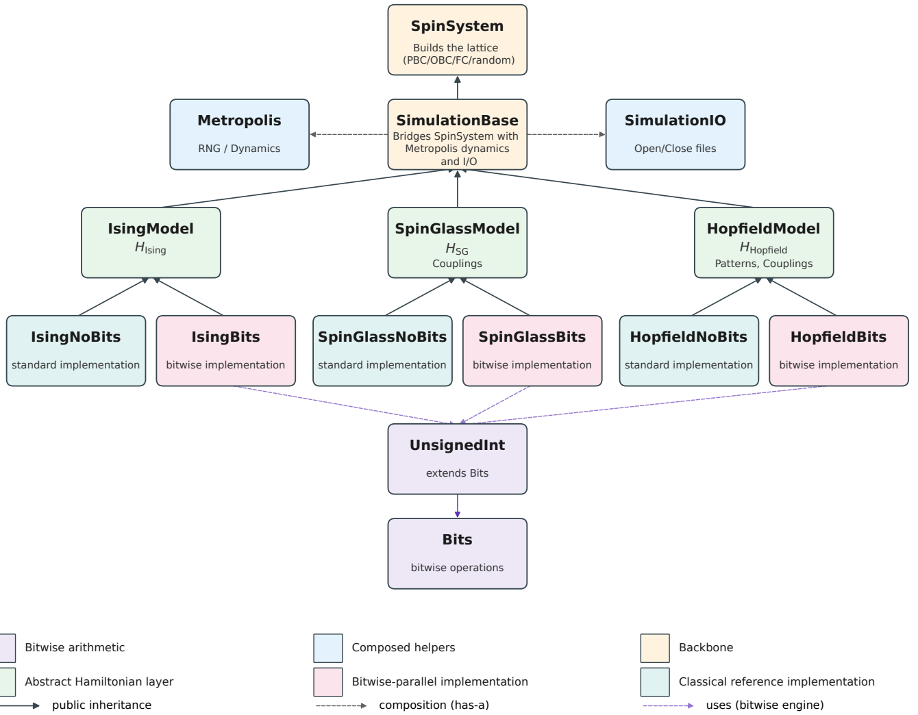
Figure 1: Code structure
