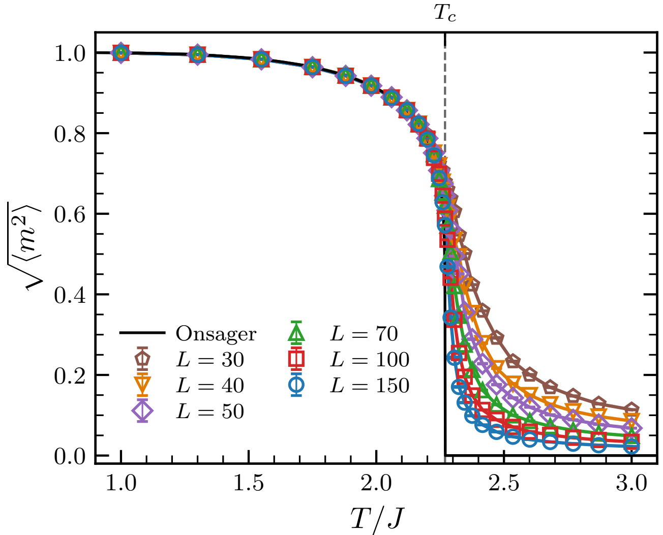
Figure 2: Phase diagram of the Ising model for several sizes of square lattices. The network is built with Periodic Boundary Conditions (PBC). The black line corresponds to the exact analytical solution found by Onsager in the case of an infinite square lattice [2]: m(T) = 0 for T \geq T_c and m(T)_{\pm} = \pm [1 - \sinh^{-4}(2K)]^{1/8} for T \leq T_c , with K = J/T and T_c/J = 2/\log(1 + \sqrt{2}) \approx 2.269 .
