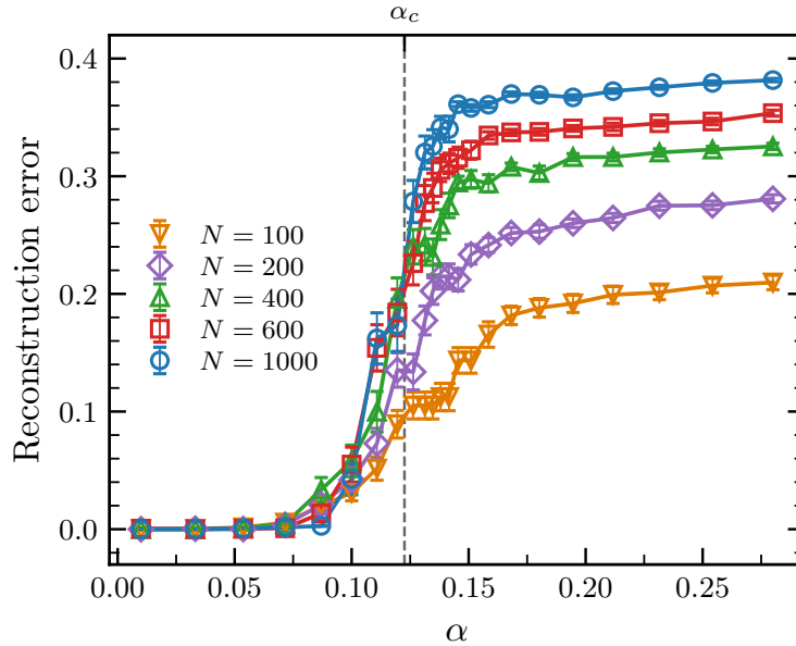
Figure 15: Evolution of the reconstruction error with the storage load for several lattice sizes. For this diagram, the configuration is initialized on one of the stored patterns.
