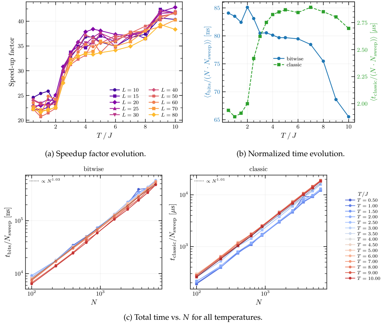
Figure 8: Performance analysis of the bitwise and classical Ising Metropolis implementations. Subfigure (a) shows the evolution of the speedup factor with the temperature for several size of square lattices. (b) shows the evolution of the normalized spin update time with the temperature, averaged over the different lattice sizes. Finally, (c) presents the evolution of the time taken to perform one sweep with the lattice size for different temperatures.
