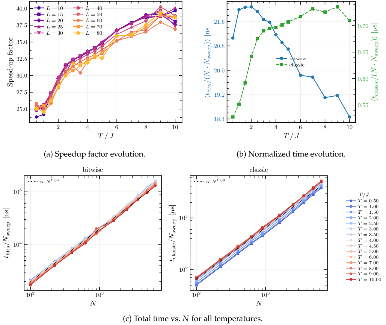
Figure 9: Performance analysis of the bitwise and classical Spin Glass Metropolis implementations.
