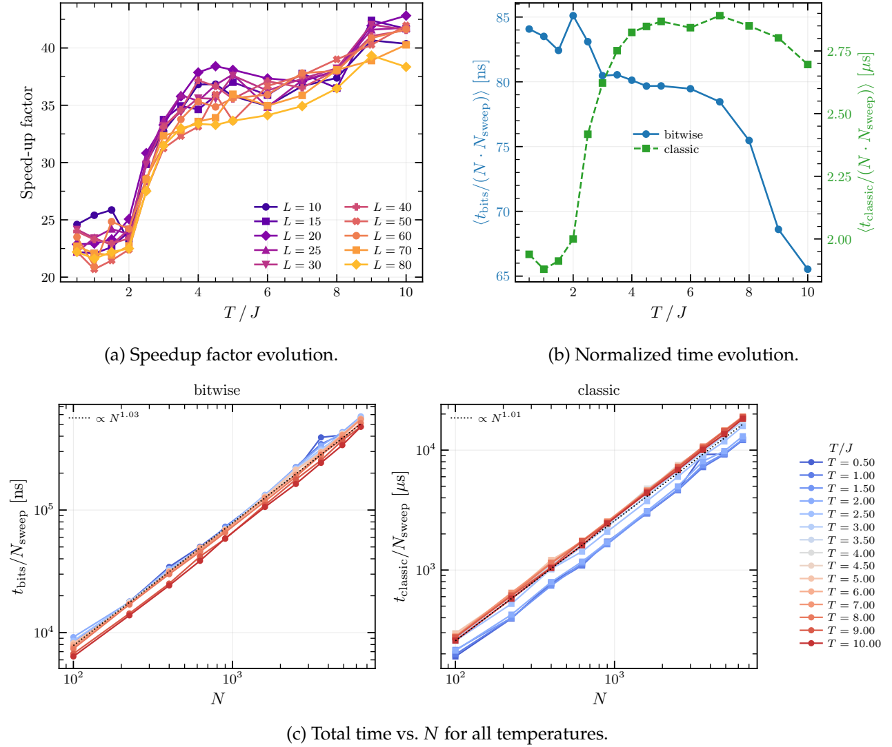
Figure 8: Performance analysis of the bitwise and classical Ising Metropolis implementations. Sub-figure (a) shows the evolution of the speedup factor with the temperature for several size of square lattices. (b) shows the evolution of the normalized spin update time with the temperature, averaged over the different lattice sizes. Finally, (c) presents the evolution of the time taken to perform one sweep with the lattice size for different temperatures.
