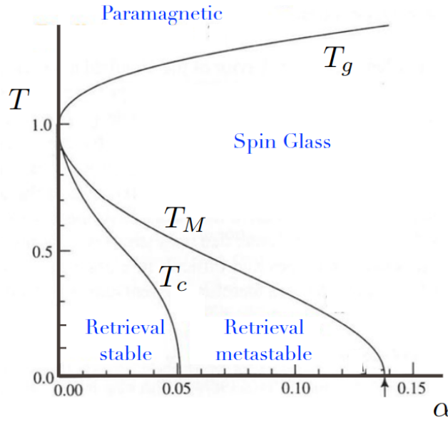
Figure 12: Phase diagram of the Hopfield model, extracted from [? ]. the phase transition value at T = 0 is signified by the arrow.
