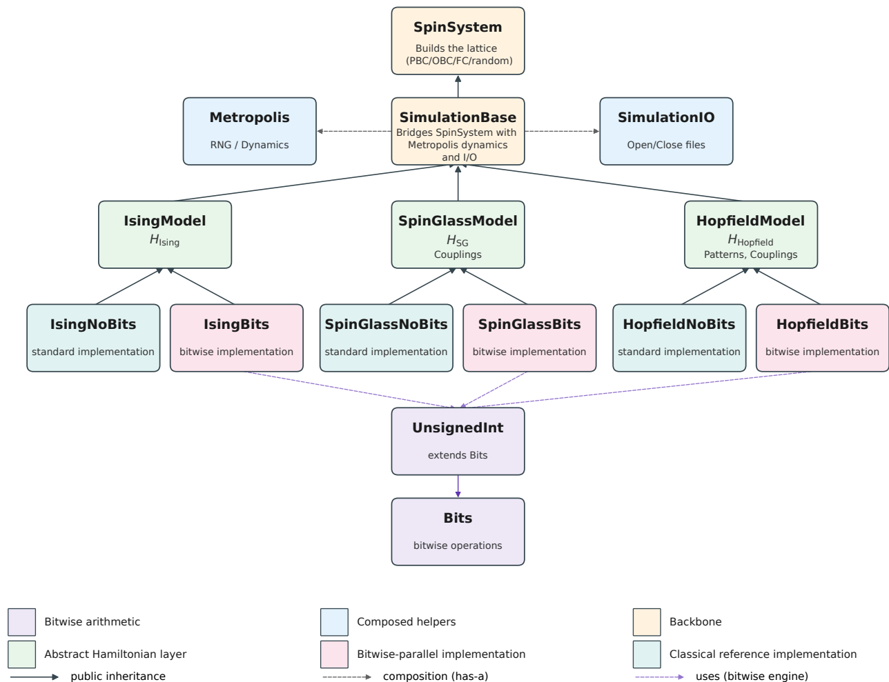
Figure 5: Code structure
