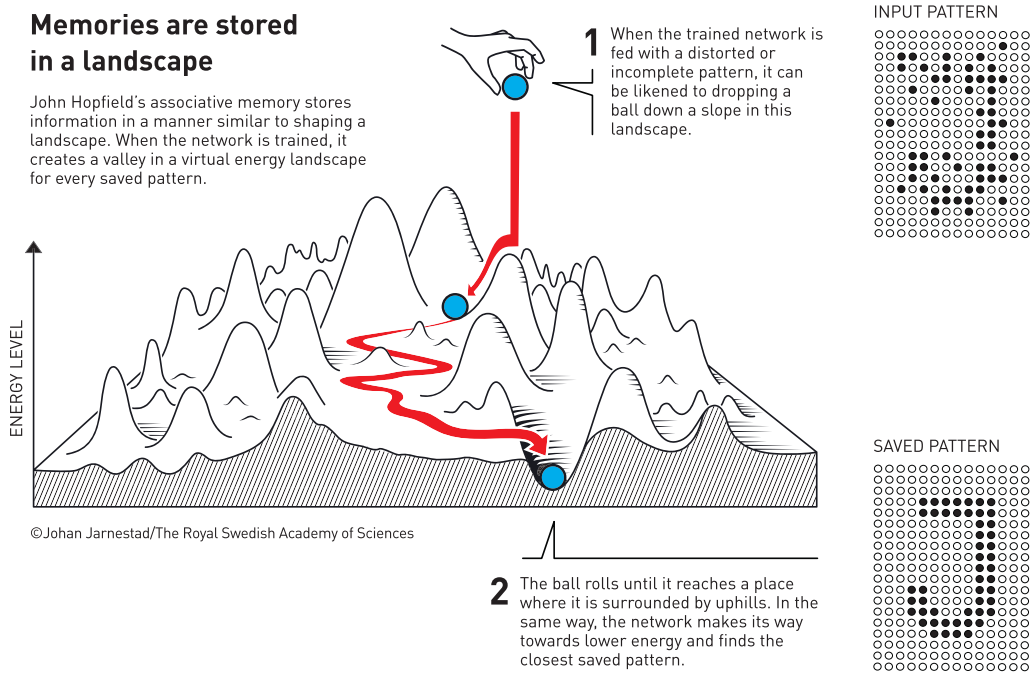
Figure 11: Schematic illustration of the Hopfield model, extracted from [? ]. The Hopfield network can recover stored patterns from an altered or partial version of them.
