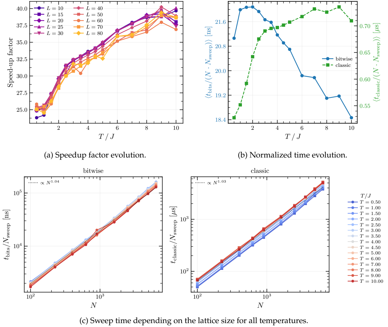
Figure 10: Performance analysis of the bitwise and classical Spin Glass Metropolis implementations.
