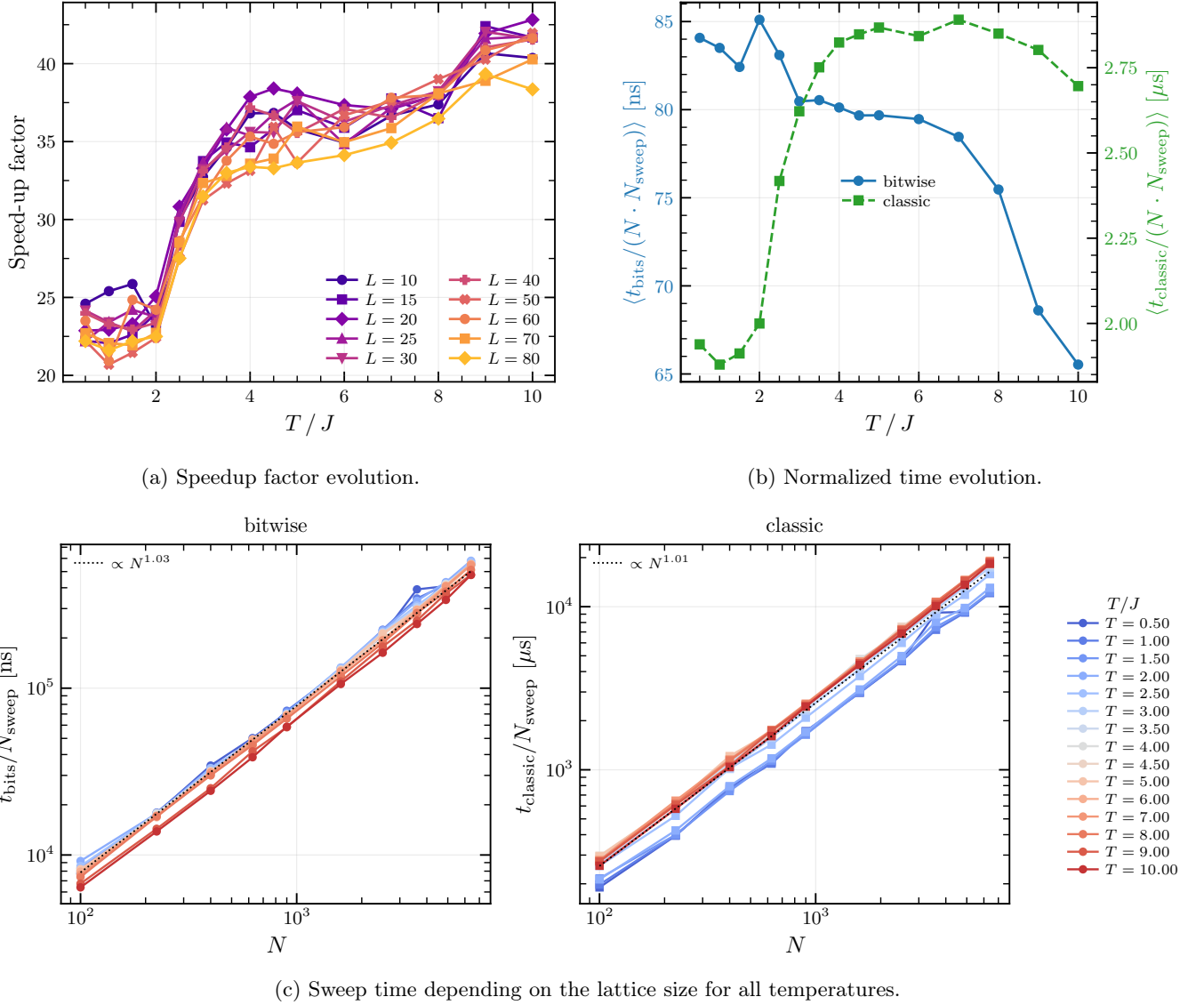
Figure 10: Performance analysis of the bitwise and classical Ising Metropolis implementations. Subfigure (a) shows the evolution of the speedup factor with the temperature for several sizes of square lattices. (b) shows the evolution of the normalized spin update time with the temperature, averaged over the different lattice sizes. Finally, (c) presents the evolution of the time taken to perform one sweep depending on the lattice size, for different temperatures.
