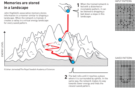
Figure 12: Schematic illustration of the Hopfield model, extracted from [1]. The Hopfield network can recover stored patterns from an altered or partial version of them.
