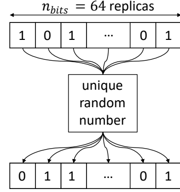
Figure 4: All 64 replicas of a given spin share the same random number at each step.
