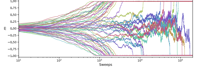
Figure 8: Trajectories of the 64 magnetizations over time for L = 100 and T/J = 1.5 . All those trajectories have been obtained from the same simulation. While some realizations quickly collapse into the equilibrium attractors m_{\pm} = \pm 0.953 , some require \sim 10^2 times more sweeps to reach the same equilibrium.
