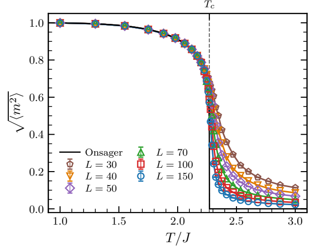
Figure 7: Phase diagram of the Ising model for several sizes of square lattices. The network is built with Periodic Boundary Conditions (PBC). The black line corresponds to the exact analytical solution found by Onsager in the case of an infinite square lattice [14]:
