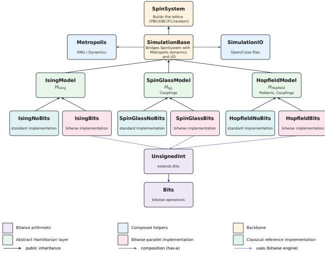
Figure 6: Code structure
