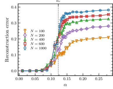
Figure 15: Evolution of the reconstruction error with the storage load for several lattice sizes. For this diagram, the configuration is initialized on one of the stored patterns.
