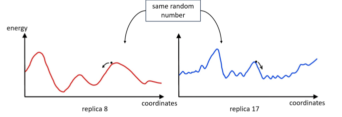
Figure 5: Schematic view of the independence of the realizations evolving from the same sequence of random numbers. Because of the unique energy landscape in every replica and the independent initializations, the same random number yields independent evolutions.
