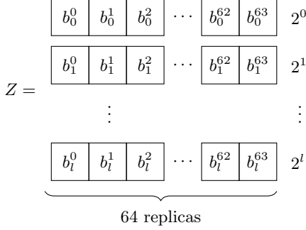
Figure 3: An UnsignedInt encoding 64 parallel unsigned integers. Each row is a Bits associated with a power of 2. The value of each integer is obtained by reading the UnsignedInt along the corresponding column. For instance, the fifth integer stored in Z is Z_4 = \sum_{i=0}^l b_i^4 2^i .
