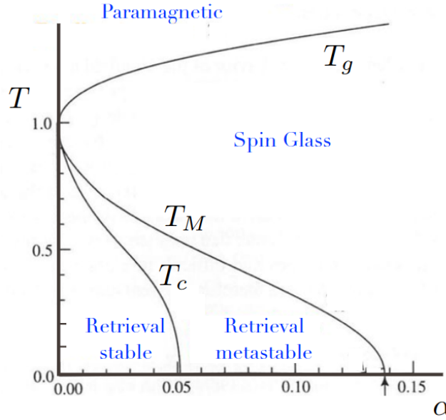
Figure 12: Phase diagram of the Hopfield model, extracted from [18].
