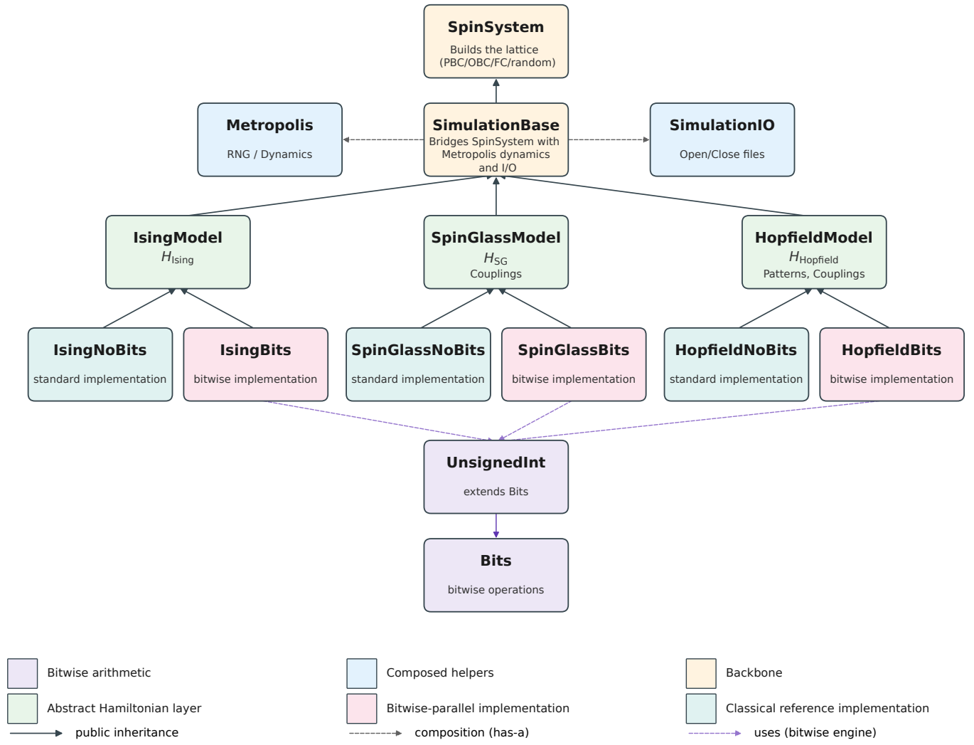
Figure 1: Code structure
