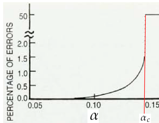
Figure 13: Evolution of the error with the storage load, extracted from [7]. For this diagram, the configuration is initialized near a pattern. When the storage load exceeds \alpha_c , the configuration becomes random and the error suddenly jumps to 0.5.
