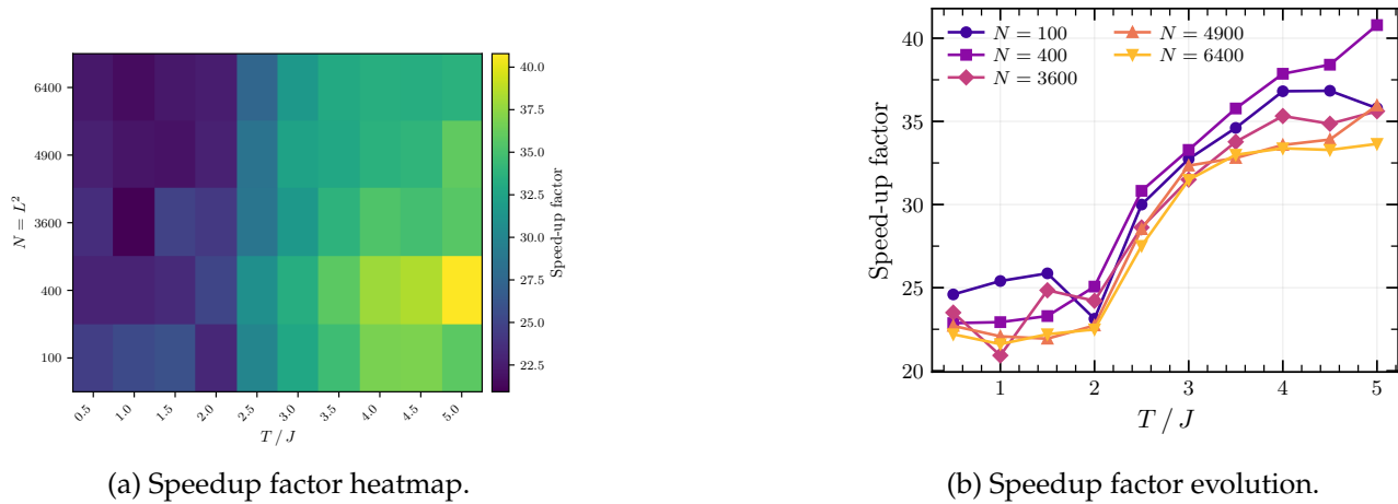
Figure 8: Speedup factor between classical and bitwise implementations of the Ising Metropolis algorithm for several lattice sizes and temperatures.
