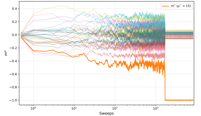
Figure 8: Evolution of m^{\mu} for all patterns for the replica 16 of \alpha = 0.03 .
