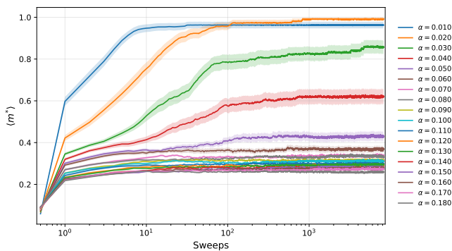
Figure 10: Evolution of \langle m^* \rangle with the storage load.
