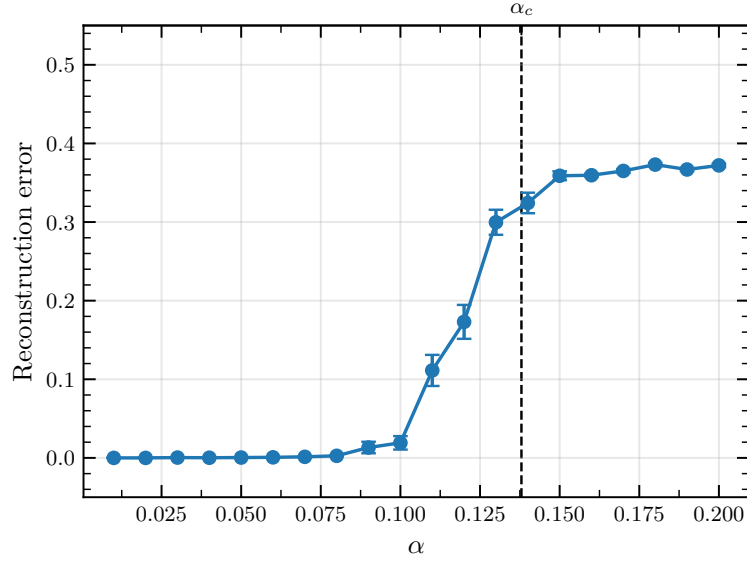
Figure 14: Evolution of the reconstruction error with the storage load. For this diagram, the configuration is initialized on a pattern.
