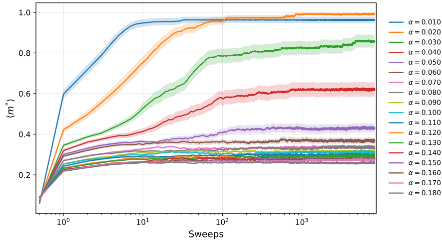
Figure 17: Evolution \langle m^* \rangle with the storage load.
