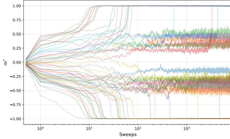
Figure 16: Evolution of the maximum overlap of each replica for \alpha = 0.03 .
