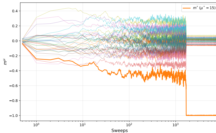
Figure 15: Evolution of m^\mu for all pattern for the replica 16 of \alpha = 0.03 .
