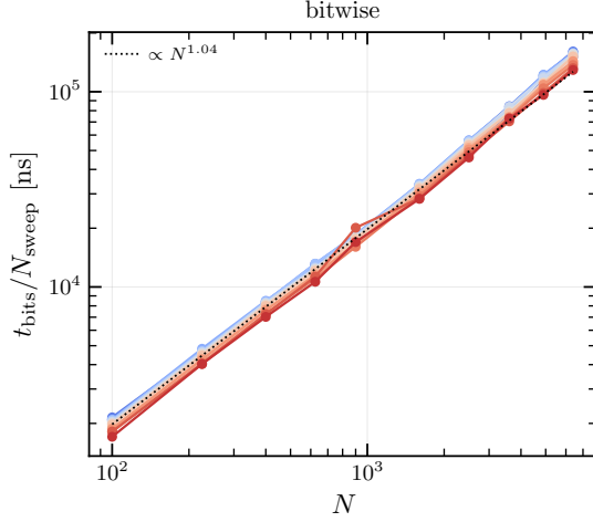
(c) Sweep time depending on the lattice size for all temperatures.
