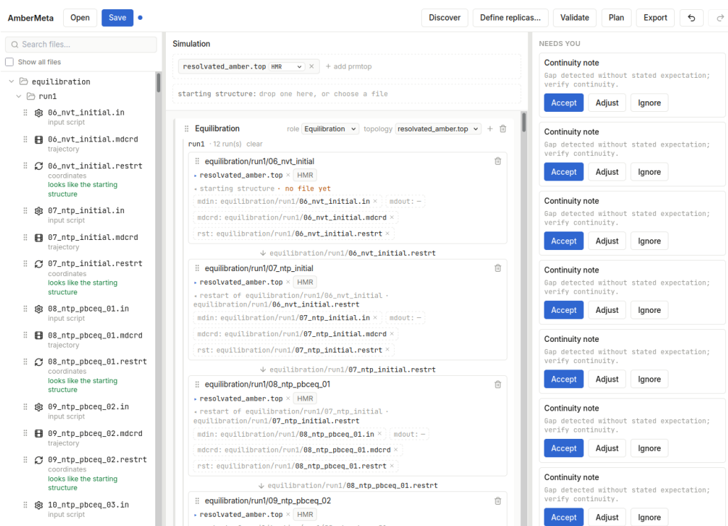
Figure 3: A system with replicas accepted: the run1 banner above the timeline marks the member and its twelve runs. The continuity notes on the right are this deposit's missing output logs — with no .mdout, no junction can be confirmed.
