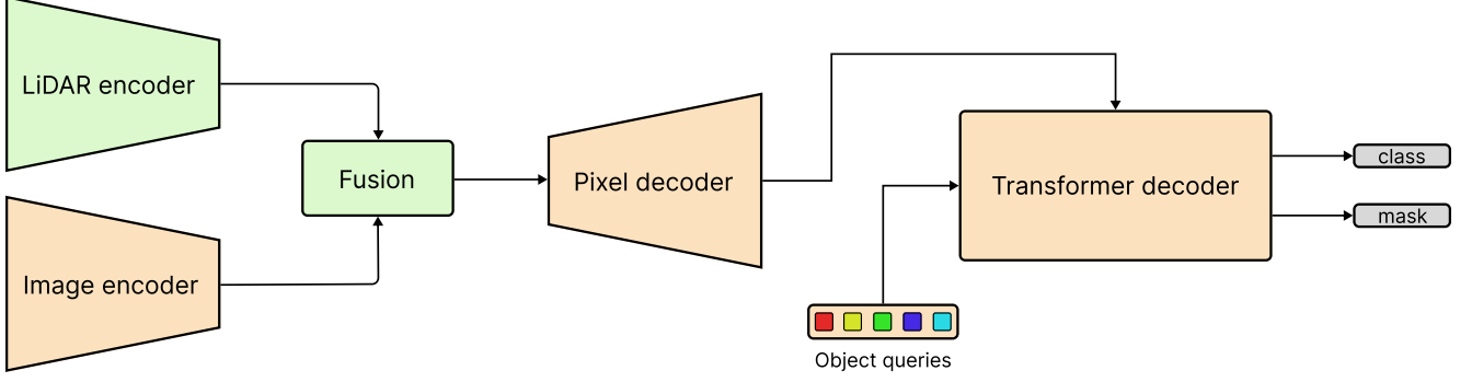
Figure 2. Overview of the proposed multimodal Mask2Former architecture. The image and LiDAR encoders generate multi-scale features with matching channels and resolutions at each level. These features are integrated within the fusion module before entering the pixel decoder. The transformer decoder refines a set of randomly initialized object queries using the fused representations to provide class and mask predictions. Modules inherited from the original Mask2Former are shown in orange, while those introduced in this work are highlighted in green.
