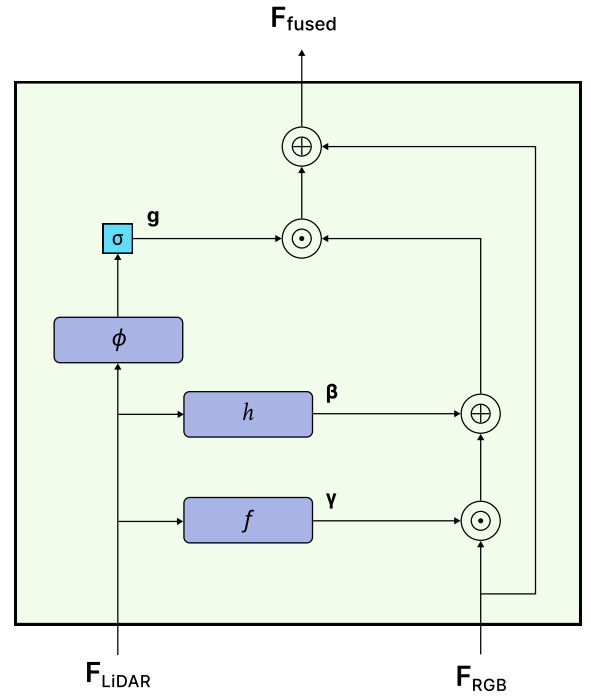
Figure 3. The feature modulation block at a given level k . Taking image ( F_{\text{RGB},k} ) and LiDAR ( F_{\text{LiDAR},k} ) features as input, the symbols \gamma_k , \beta_k , and g_k denote the scale, shift, and gating tensors, respectively. The functions f , h , and \phi represent 1 \times 1 convolutions, while \sigma indicates the sigmoid activation. The symbols \oplus and \odot indicate element-wise addition and the Hadamard product.
