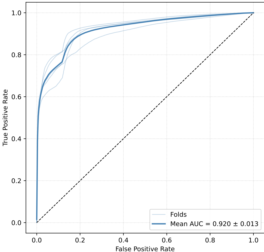
RTBM ROC — N_h=2 , 5-fold
