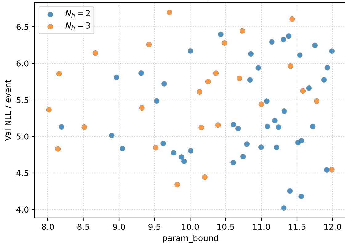
NLL vs param_bound
