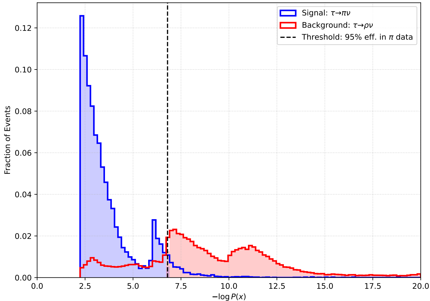
RTBM: Anomaly Scores ( -\log P(x) )
