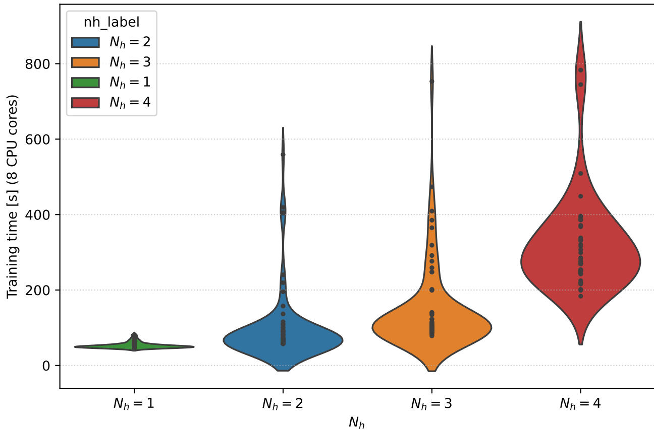
Training time vs N_h (250 CMA iterations)
