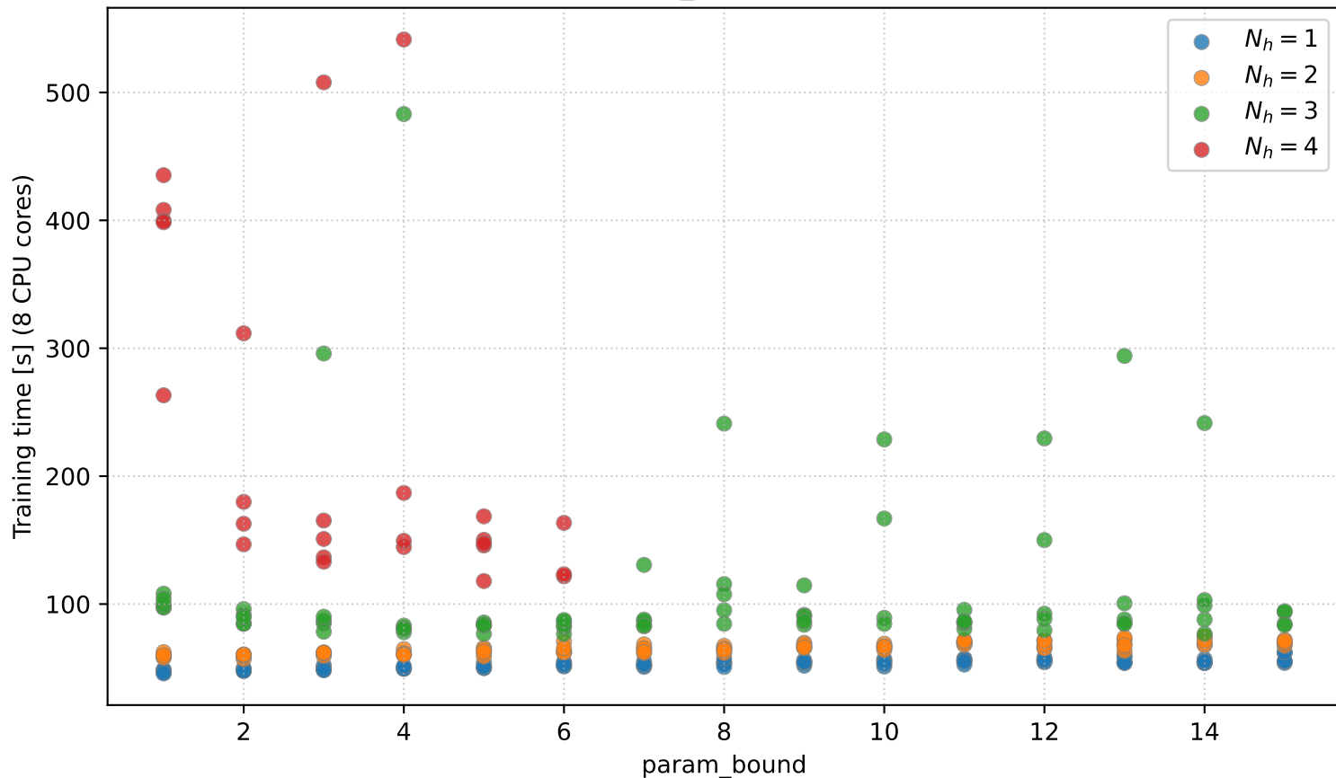
Training time vs param_bound (250 CMA iterations)
