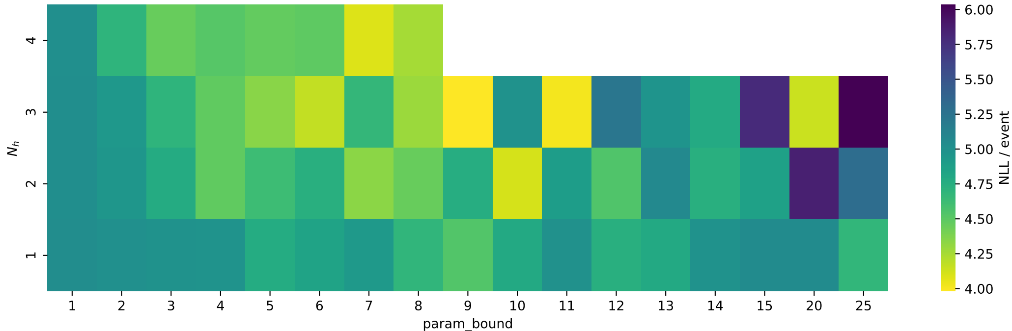
RTBM: Mean VAL NLL - 5 runs , 250 maxiter
